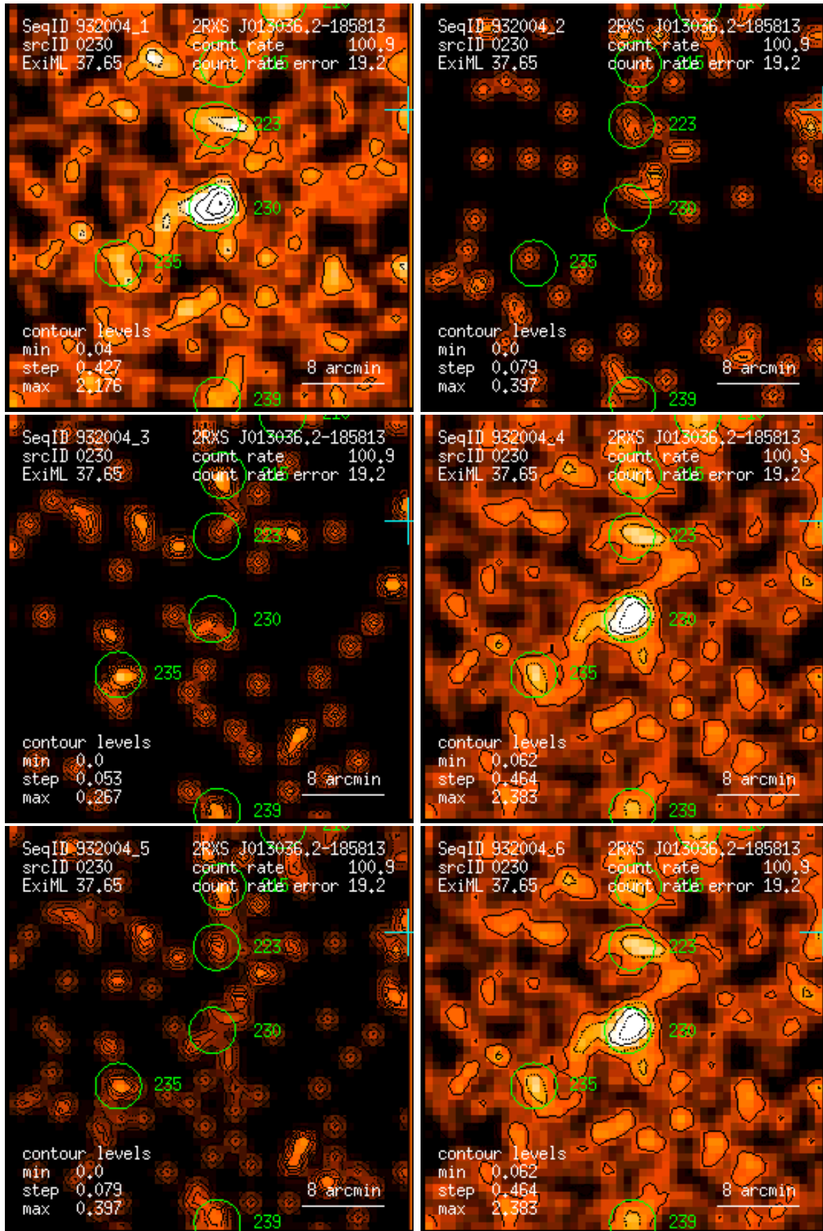
Figure 230: RASS 932004: detection 0230: band rate images, Gaussian filter: (1) PSPC channels 11 – 41, (2) 52 – 90, (3) 91 – 201, (4) 11 – 235, (5) 52 – 201, (6) 11 – 201. Broad band rates in counts/ks. Band rate contour levels in counts/ks/arcmin 2 .
