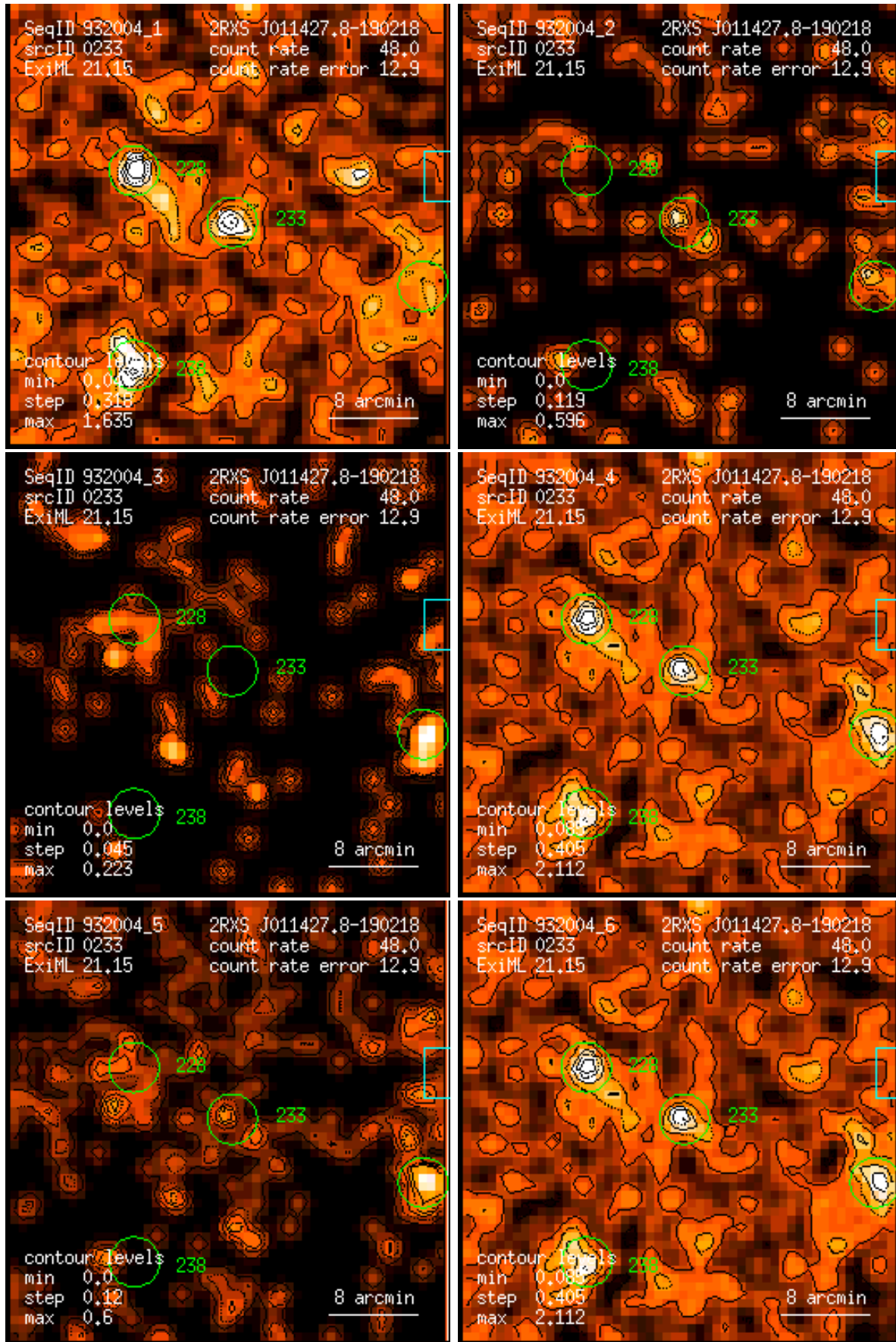
Figure 233: RASS 932004: detection 0233: band rate images, Gaussian filter: (1) PSPC channels 11 – 41, (2) 52 – 90, (3) 91 – 201, (4) 11 – 235, (5) 52 – 201, (6) 11 – 201. Broad band rates in counts/ks. Band rate contour levels in counts/ks/arcmin 2 .
