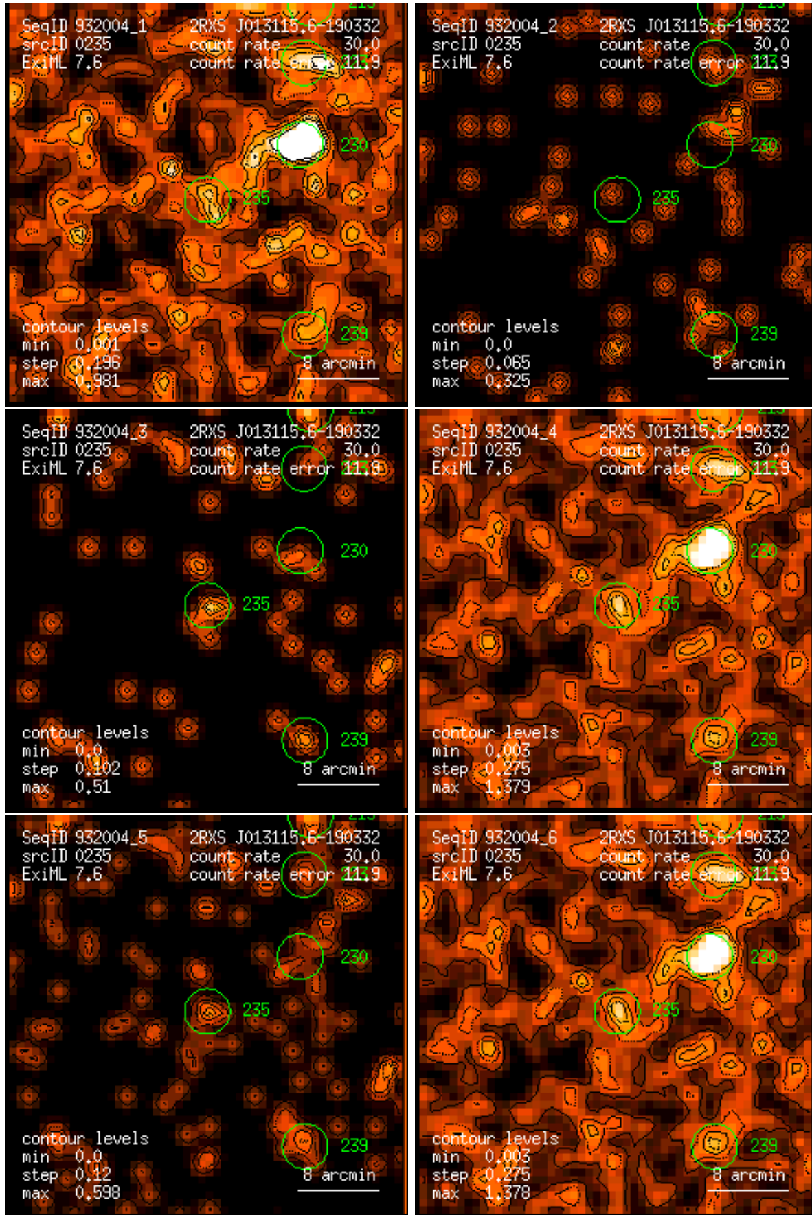
Figure 235: RASS 932004: detection 0235: band rate images, Gaussian filter: (1) PSPC channels 11 – 41, (2) 52 – 90, (3) 91 – 201, (4) 11 – 235, (5) 52 – 201, (6) 11 – 201. Broad band rates in counts/ks. Band rate contour levels in counts/ks/arcmin 2 .
