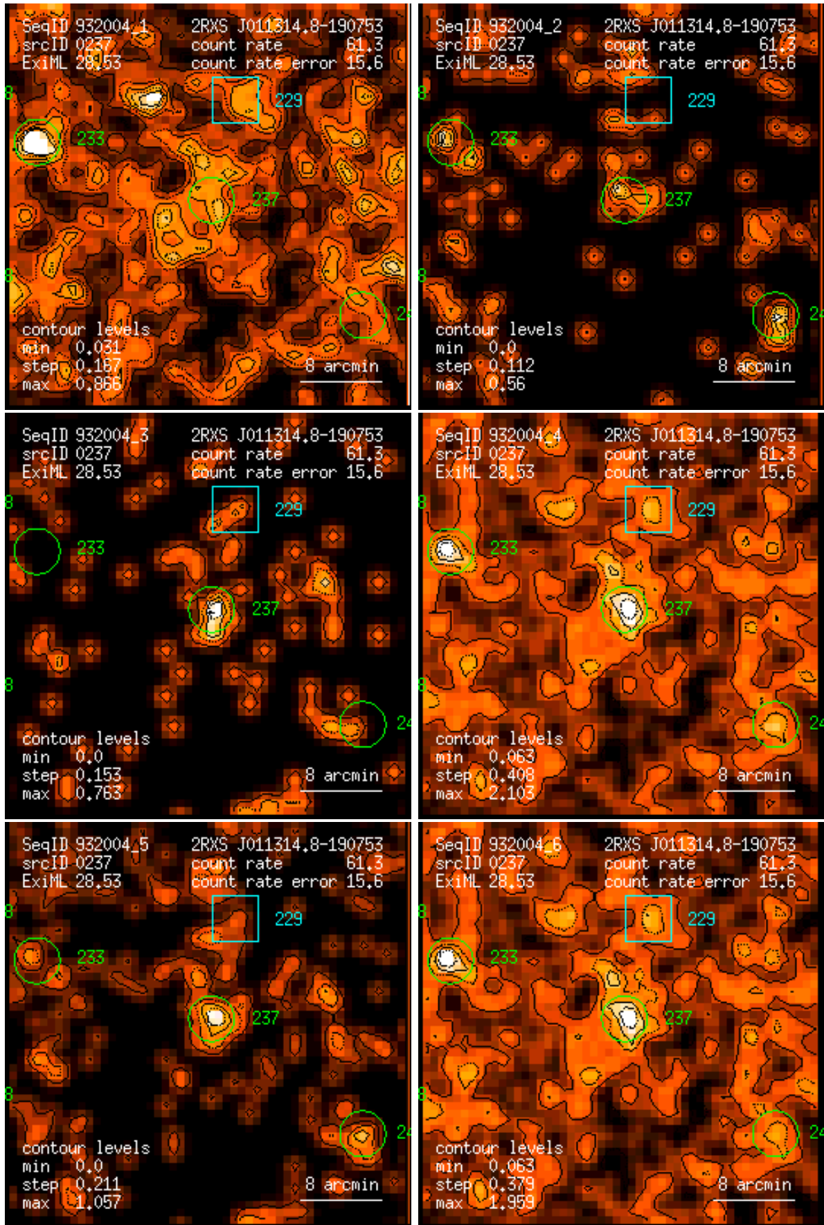
Figure 237: RASS 932004: detection 0237: band rate images, Gaussian filter: (1) PSPC channels 11 – 41, (2) 52 – 90, (3) 91 – 201, (4) 11 – 235, (5) 52 – 201, (6) 11 – 201. Broad band rates in counts/ks. Band rate contour levels in counts/ks/arcmin 2 .
