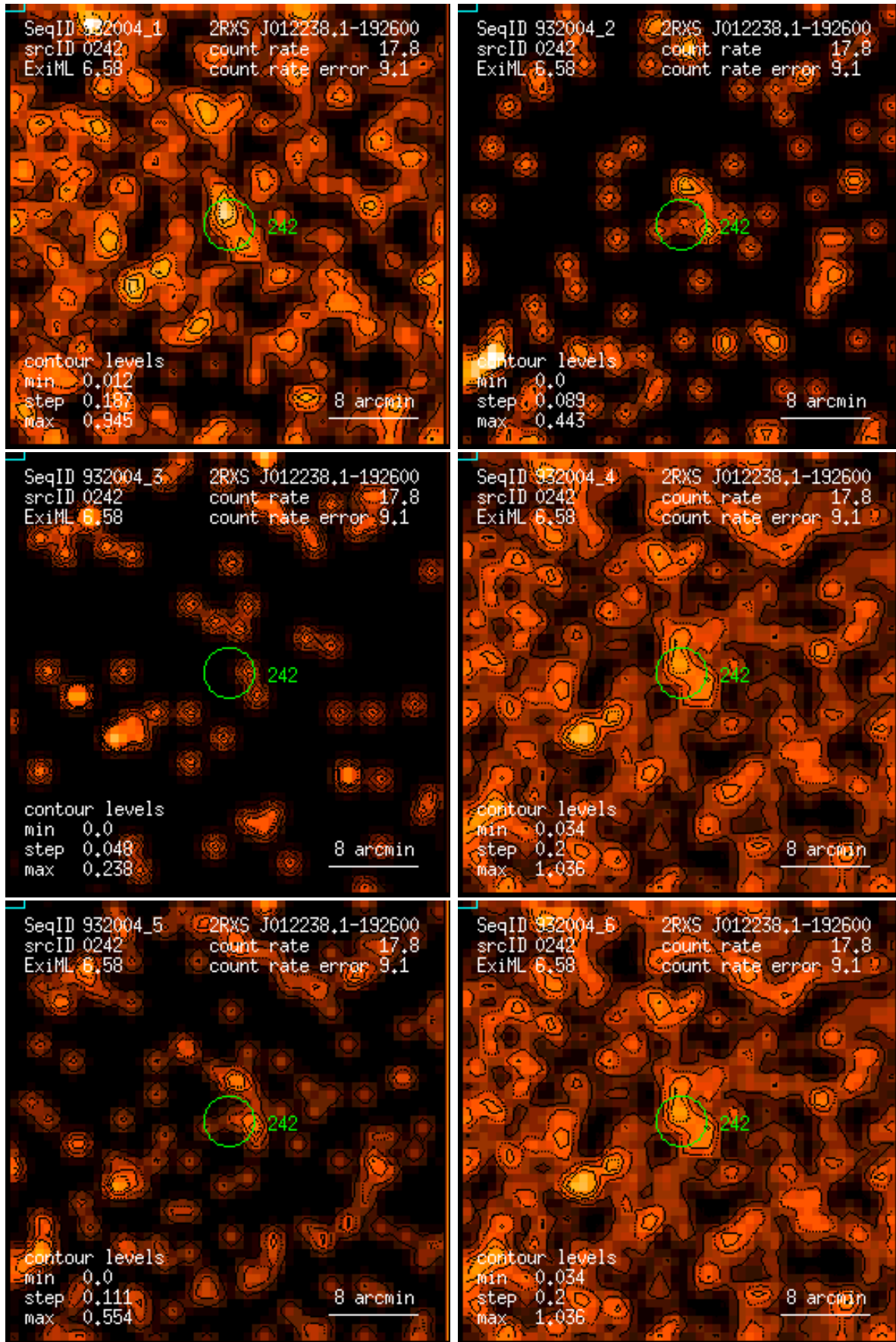
Figure 242: RASS 932004: detection 0242: band rate images, Gaussian filter: (1) PSPC channels 11 – 41, (2) 52 – 90, (3) 91 – 201, (4) 11 – 235, (5) 52 – 201, (6) 11 – 201. Broad band rates in counts/ks. Band rate contour levels in counts/ks/arcmin 2 .
