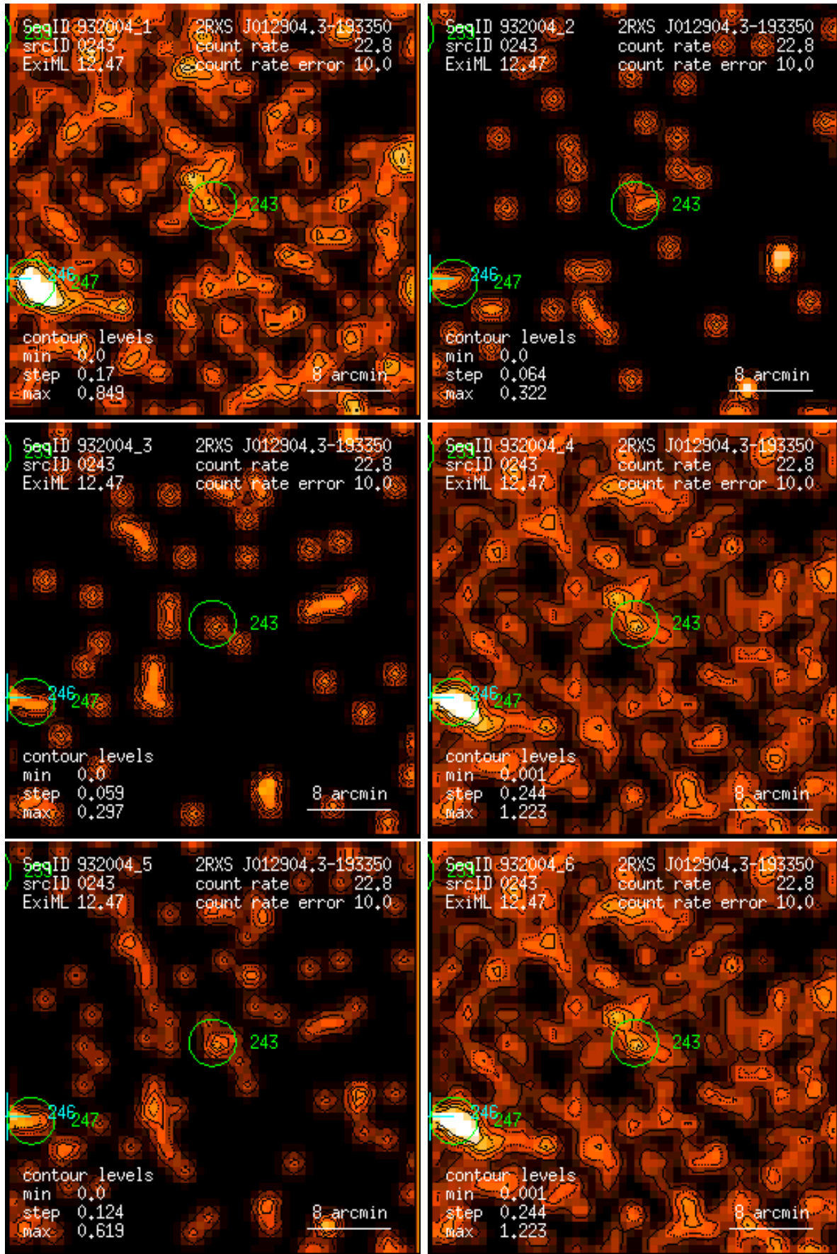
Figure 243: RASS 932004: detection 0243: band rate images, Gaussian filter: (1) PSPC channels 11 – 41, (2) 52 – 90, (3) 91 – 201, (4) 11 – 235, (5) 52 – 201, (6) 11 – 201. Broad band rates in counts/ks. Band rate contour levels in counts/ks/arcmin 2 .
