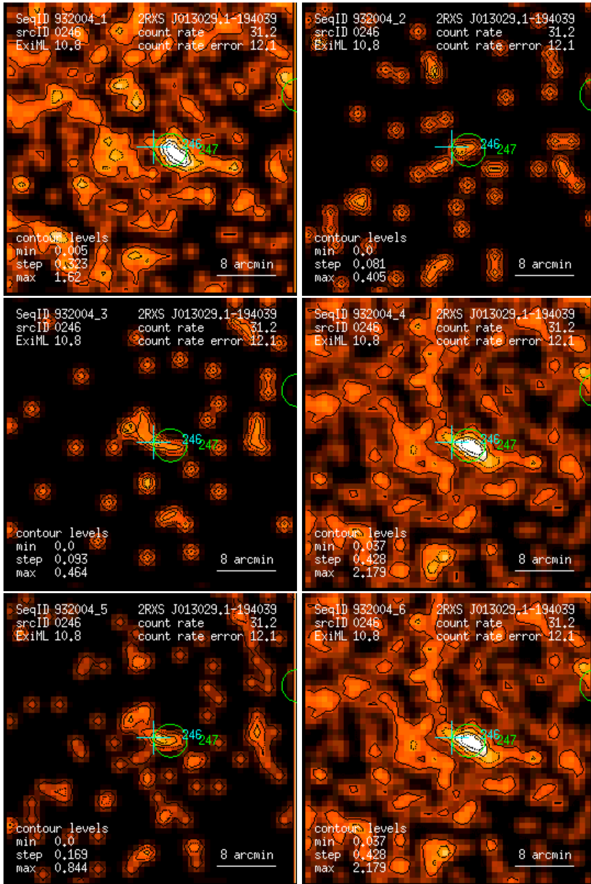
Figure 246: RASS 932004: detection 0246: band rate images, Gaussian filter: (1) PSPC channels 11 – 41, (2) 52 – 90, (3) 91 – 201, (4) 11 – 235, (5) 52 – 201, (6) 11 – 201. Broad band rates in counts/ks. Band rate contour levels in counts/ks/arcmin 2 .
