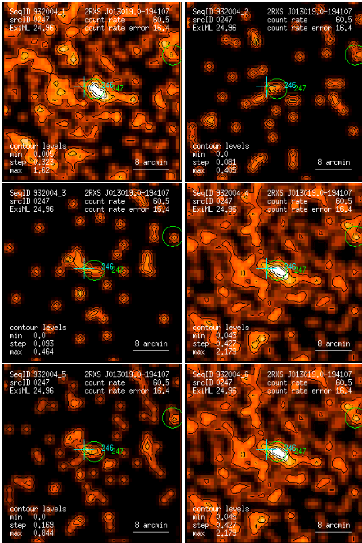
Figure 247: RASS 932004: detection 0247: band rate images, Gaussian filter: (1) PSPC channels 11 – 41, (2) 52 – 90, (3) 91 – 201, (4) 11 – 235, (5) 52 – 201, (6) 11 – 201. Broad band rates in counts/ks. Band rate contour levels in counts/ks/arcmin 2 .
