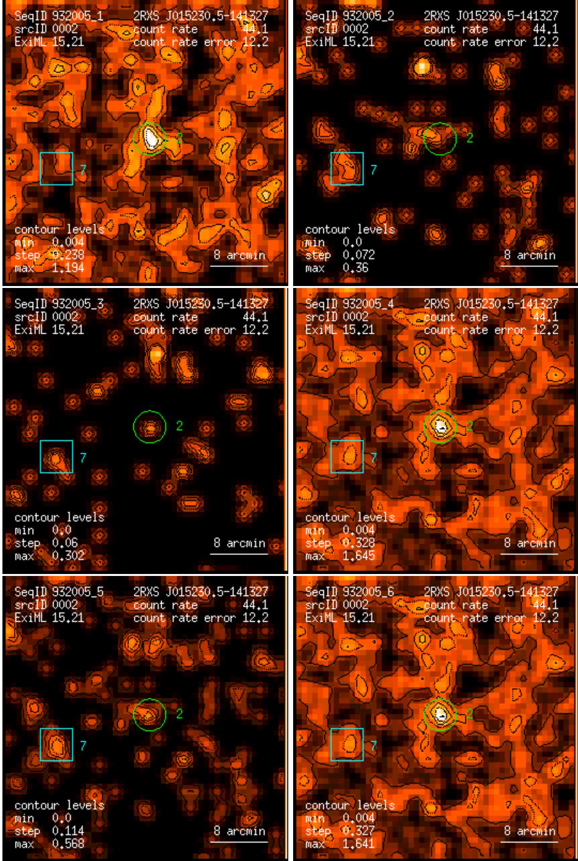
Figure 2: RASS 932005: detection 0002: band rate images, Gaussian filter: (1) PSPC channels 11 – 41, (2) 52 – 90, (3) 91 – 201, (4) 11 – 235, (5) 52 – 201, (6) 11 – 201. Broad band rates in counts/ks. Band rate contour levels in counts/ks/arcmin 2 .
