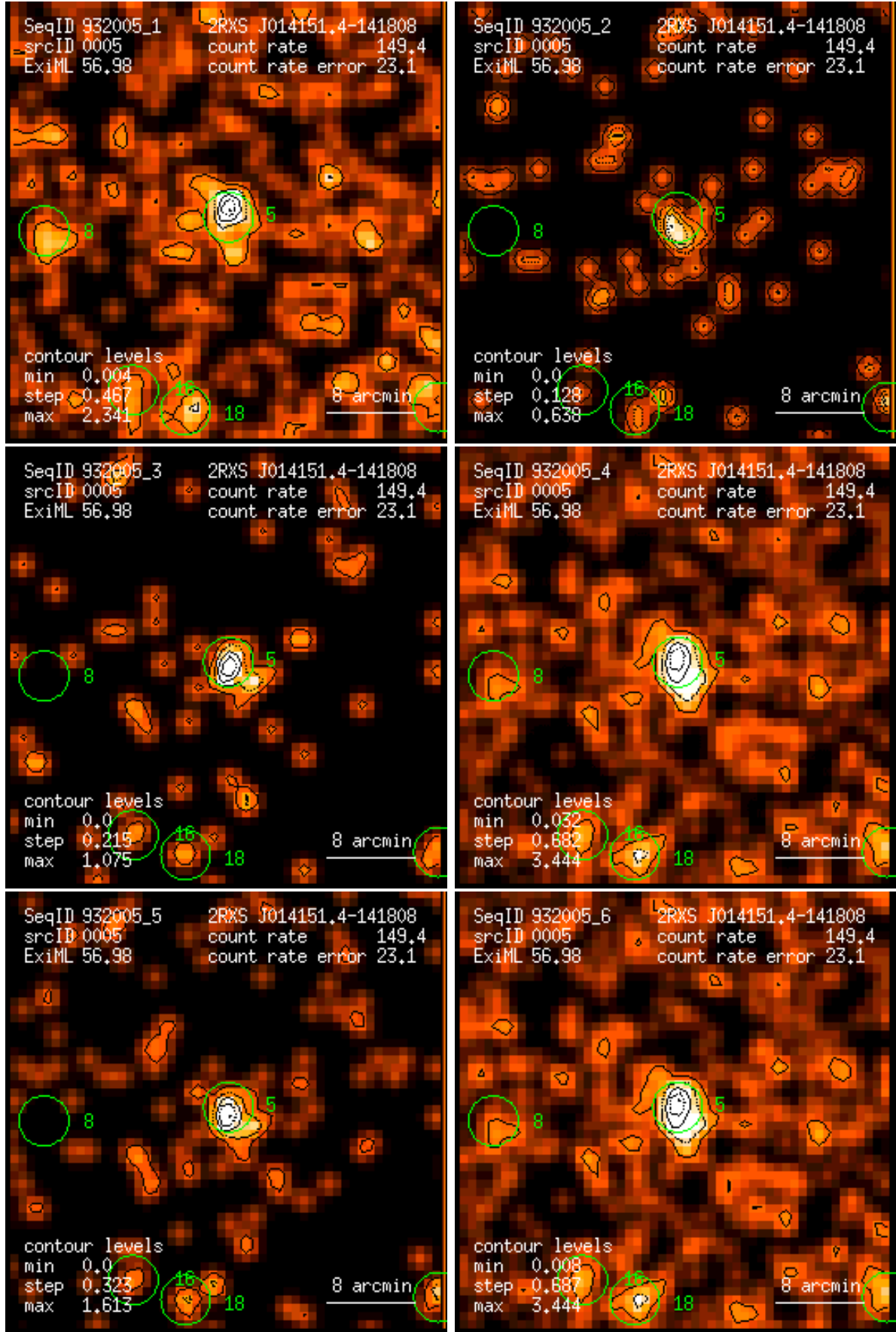
Figure 5: RASS 932005: detection 0005: band rate images, Gaussian filter: (1) PSPC channels 11 – 41, (2) 52 – 90, (3) 91 – 201, (4) 11 – 235, (5) 52 – 201, (6) 11 – 201. Broad band rates in counts/ks. Band rate contour levels in counts/ks/arcmin 2 .
