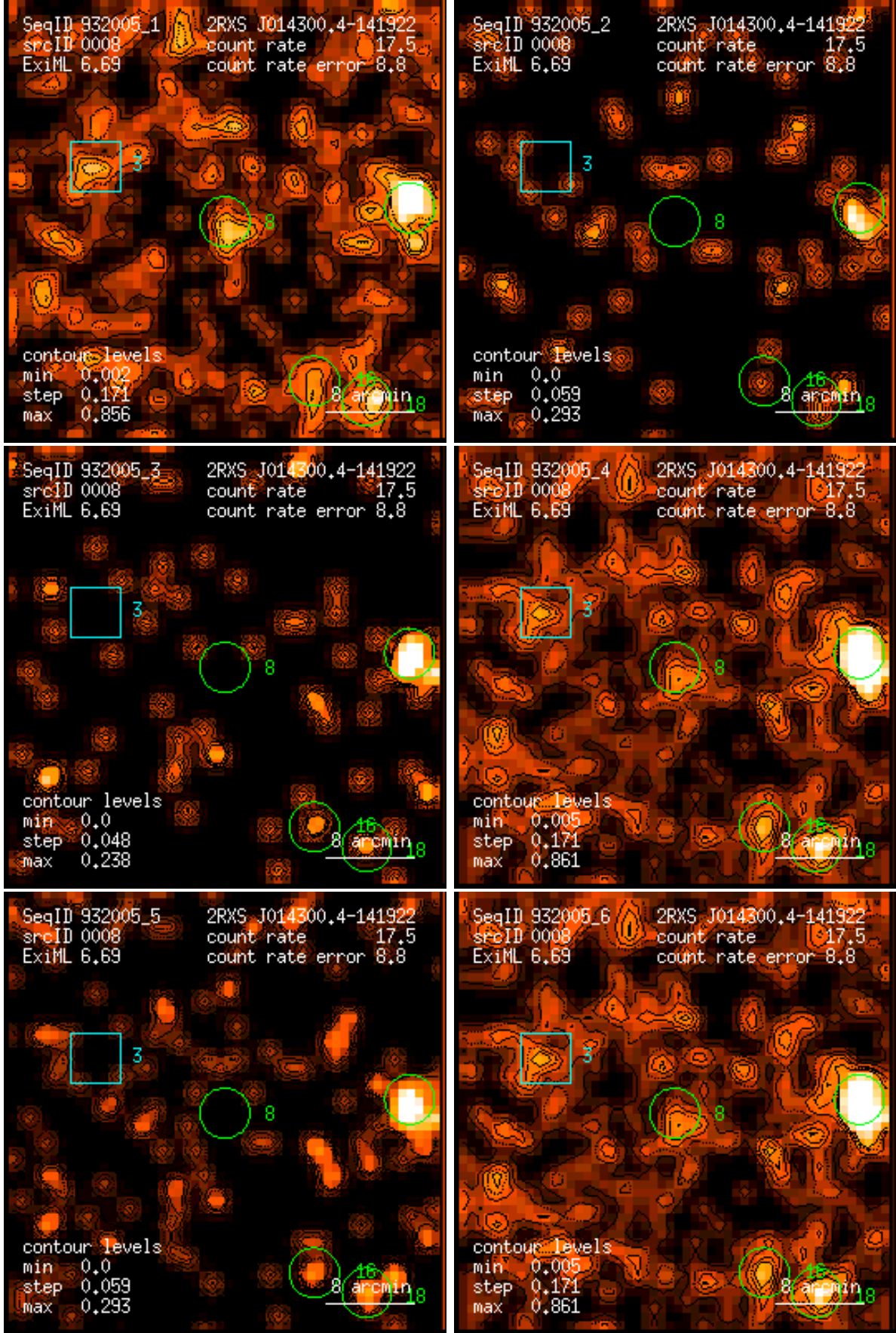
Figure 8: RASS 932005: detection 0008: band rate images, Gaussian filter: (1) PSPC channels 11 – 41, (2) 52 – 90, (3) 91 – 201, (4) 11 – 235, (5) 52 – 201, (6) 11 – 201. Broad band rates in counts/ks. Band rate contour levels in counts/ks/arcmin 2 .
