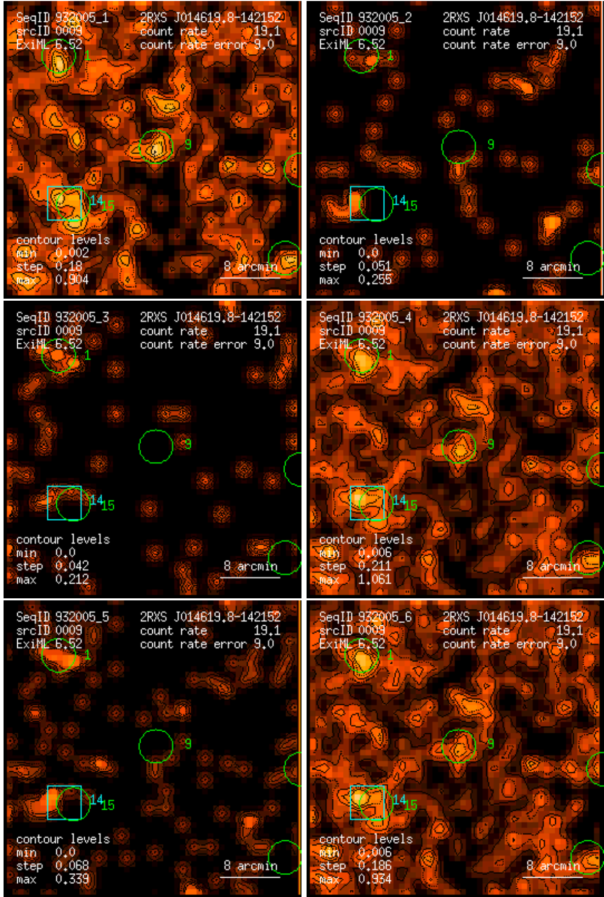
Figure 9: RASS 932005: detection 0009: band rate images, Gaussian filter: (1) PSPC channels 11 – 41, (2) 52 – 90, (3) 91 – 201, (4) 11 – 235, (5) 52 – 201, (6) 11 – 201. Broad band rates in counts/ks. Band rate contour levels in counts/ks/arcmin 2 .
