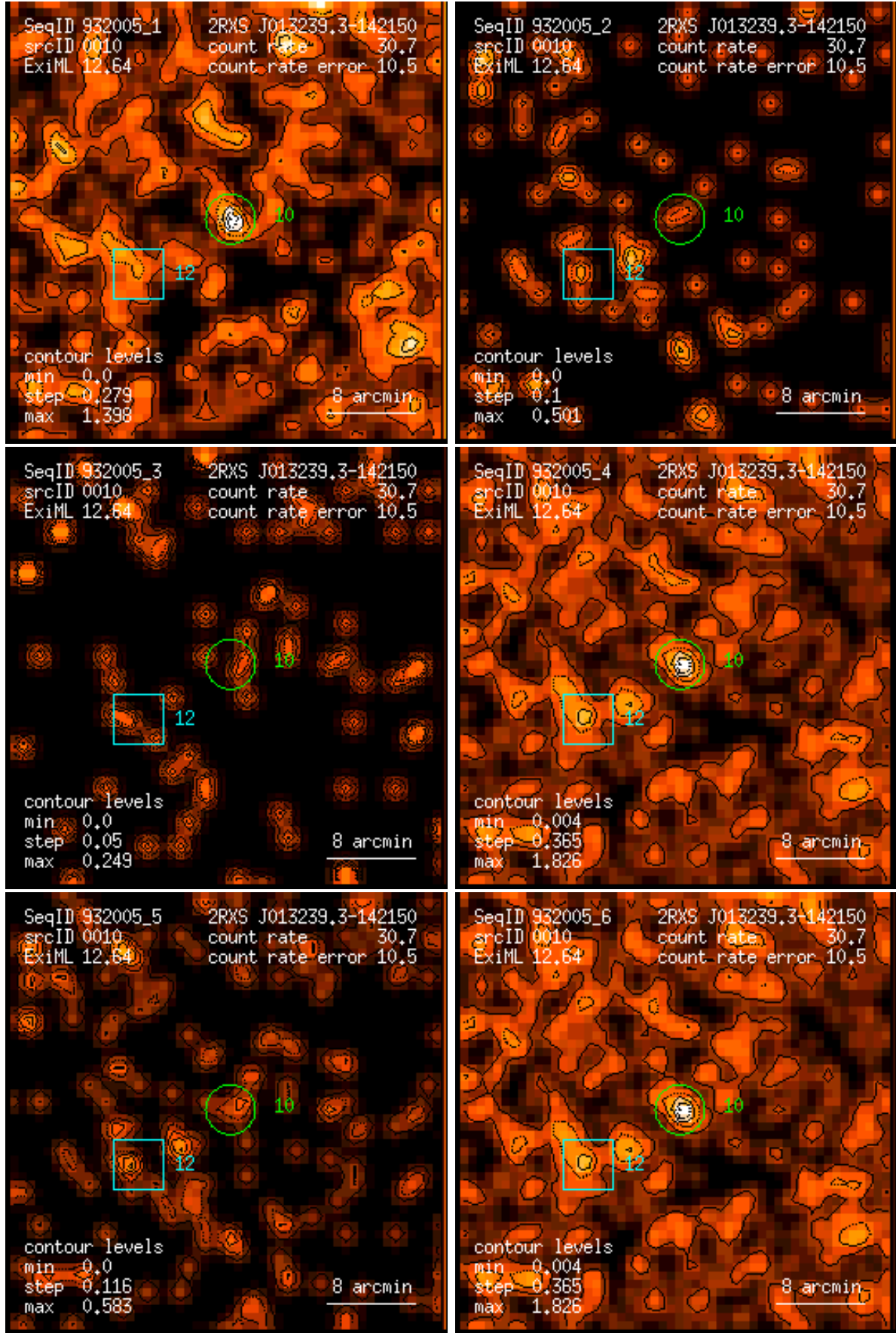
Figure 10: RASS 932005: detection 0010: band rate images, Gaussian filter: (1) PSPC channels 11 – 41, (2) 52 – 90, (3) 91 – 201, (4) 11 – 235, (5) 52 – 201, (6) 11 – 201. Broad band rates in counts/ks. Band rate contour levels in counts/ks/arcmin 2 .
