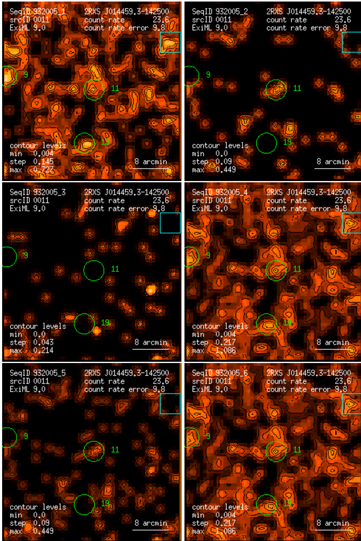
Figure 11: RASS 932005: detection 0011: band rate images, Gaussian filter: (1) PSPC channels 11 – 41, (2) 52 – 90, (3) 91 – 201, (4) 11 – 235, (5) 52 – 201, (6) 11 – 201. Broad band rates in counts/ks. Band rate contour levels in counts/ks/arcmin 2 .
