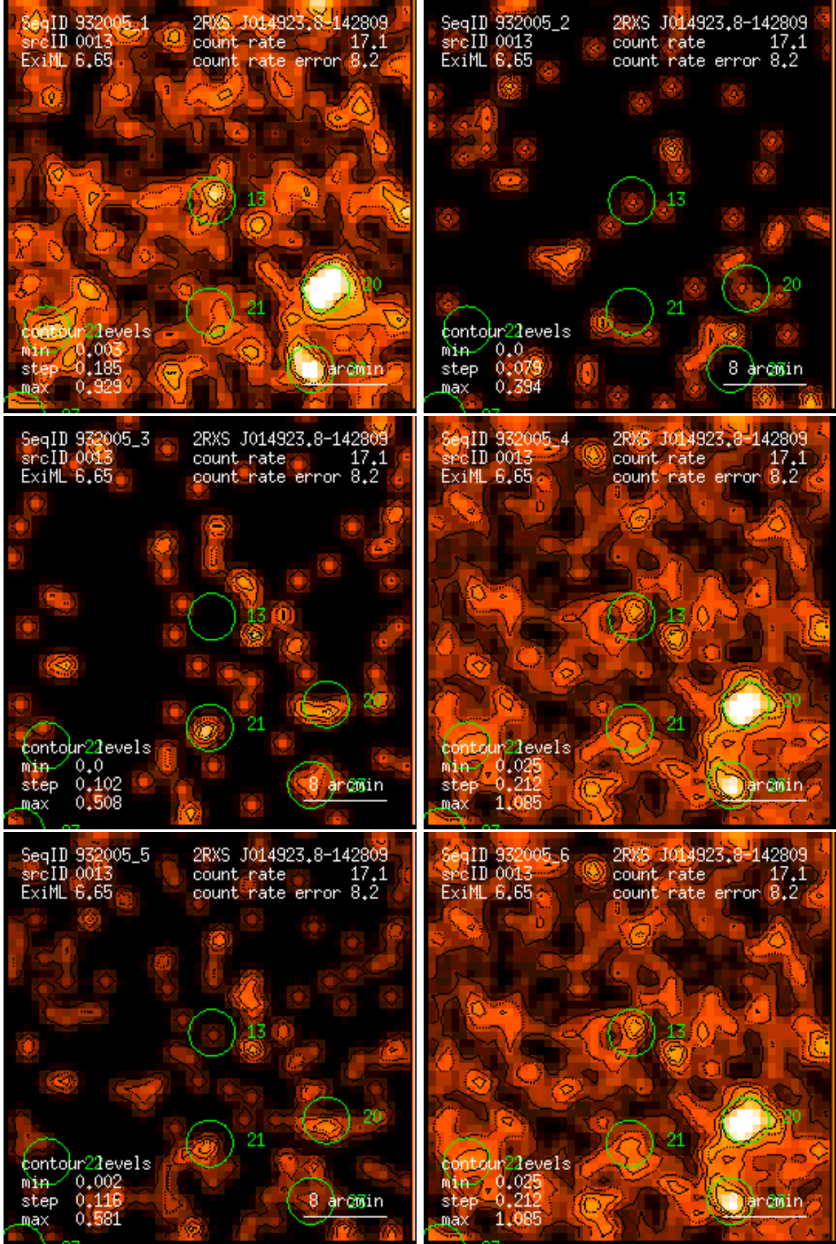
Figure 13: RASS 932005: detection 0013: band rate images, Gaussian filter: (1) PSPC channels 11 – 41, (2) 52 – 90, (3) 91 – 201, (4) 11 – 235, (5) 52 – 201, (6) 11 – 201. Broad band rates in counts/ks. Band rate contour levels in counts/ks/arcmin 2 .
