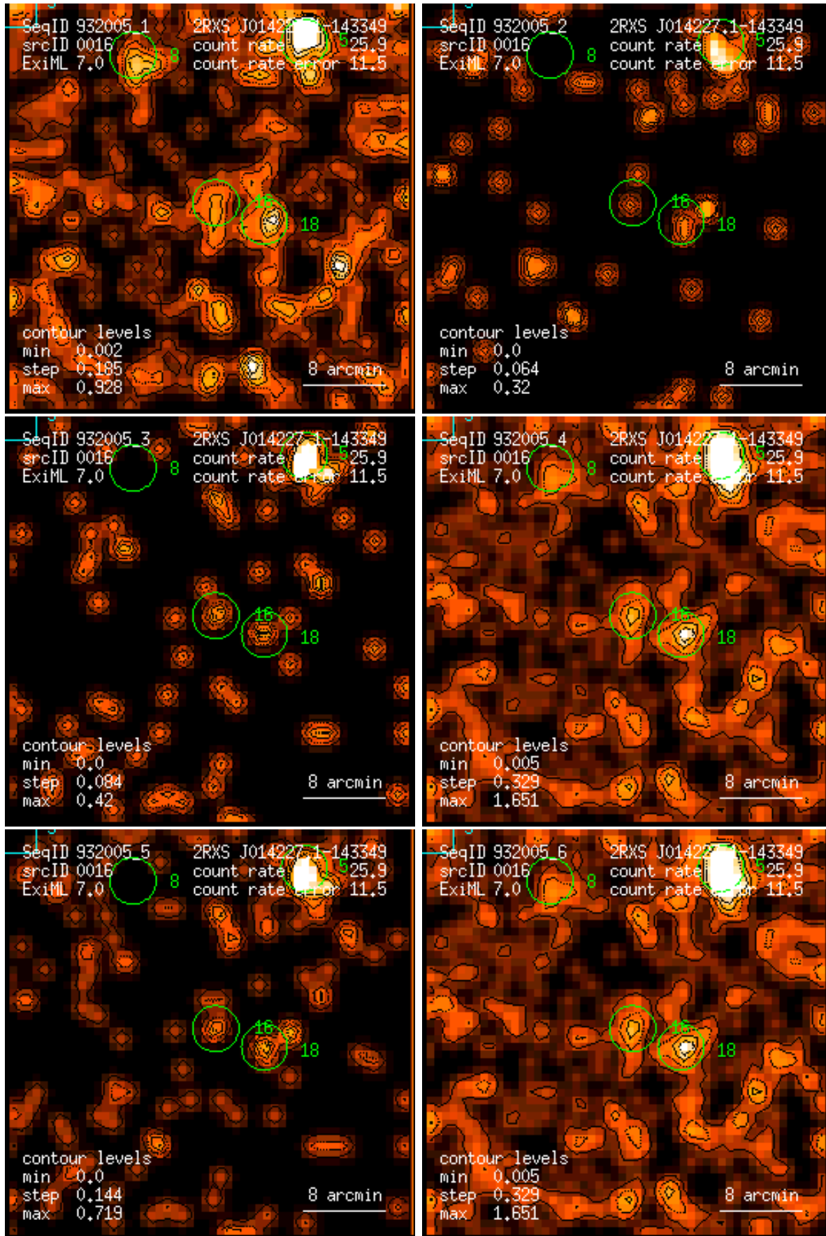
Figure 16: RASS 932005: detection 0016: band rate images, Gaussian filter: (1) PSPC channels 11 – 41, (2) 52 – 90, (3) 91 – 201, (4) 11 – 235, (5) 52 – 201, (6) 11 – 201. Broad band rates in counts/ks. Band rate contour levels in counts/ks/arcmin 2 .
