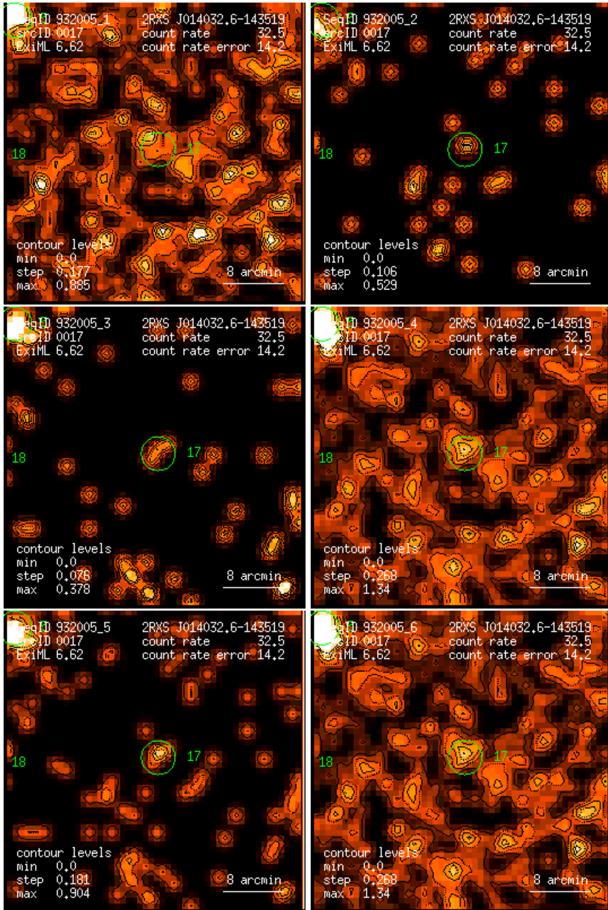
Figure 17: RASS 932005: detection 0017: band rate images, Gaussian filter: (1) PSPC channels 11 – 41, (2) 52 – 90, (3) 91 – 201, (4) 11 – 235, (5) 52 – 201, (6) 11 – 201. Broad band rates in counts/ks. Band rate contour levels in counts/ks/arcmin 2 .
