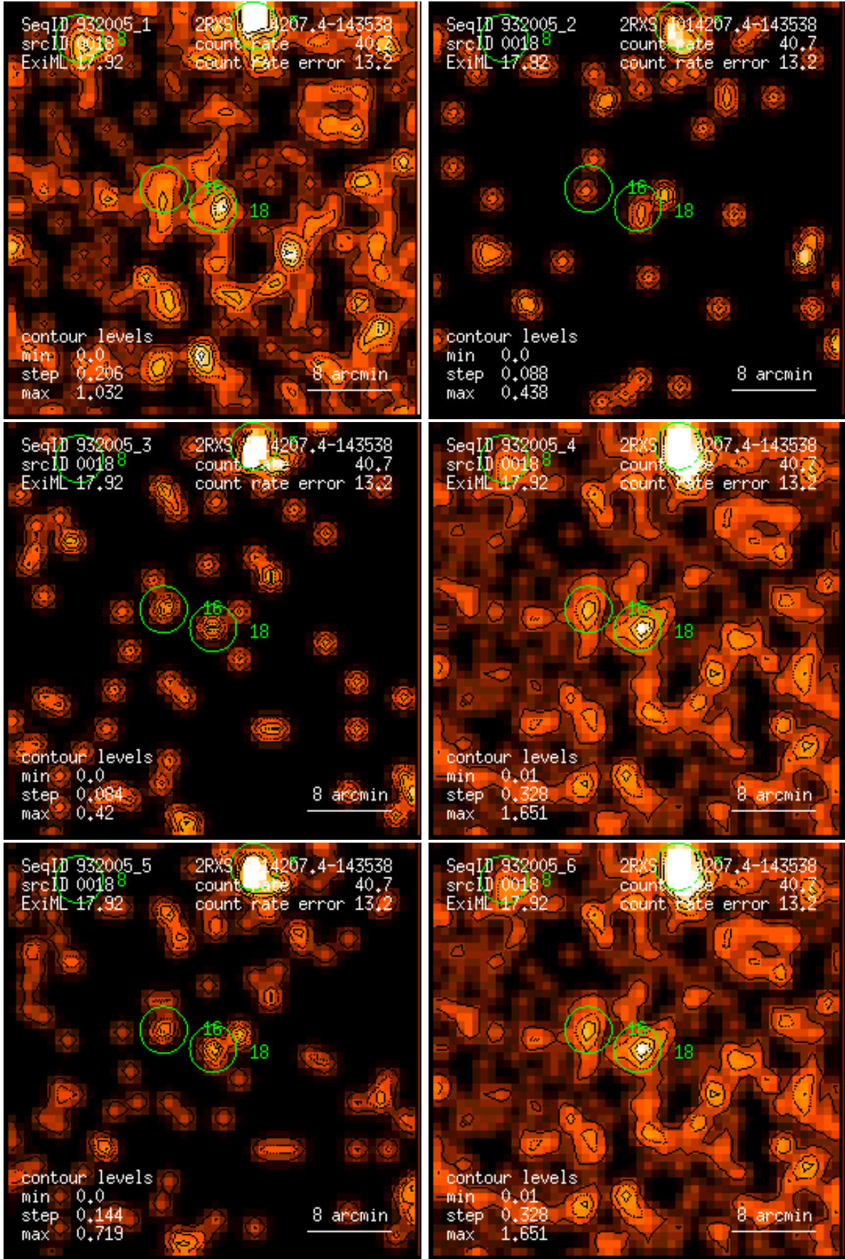
Figure 18: RASS 932005: detection 0018: band rate images, Gaussian filter: (1) PSPC channels 11 – 41, (2) 52 – 90, (3) 91 – 201, (4) 11 – 235, (5) 52 – 201, (6) 11 – 201. Broad band rates in counts/ks. Band rate contour levels in counts/ks/arcmin 2 .
