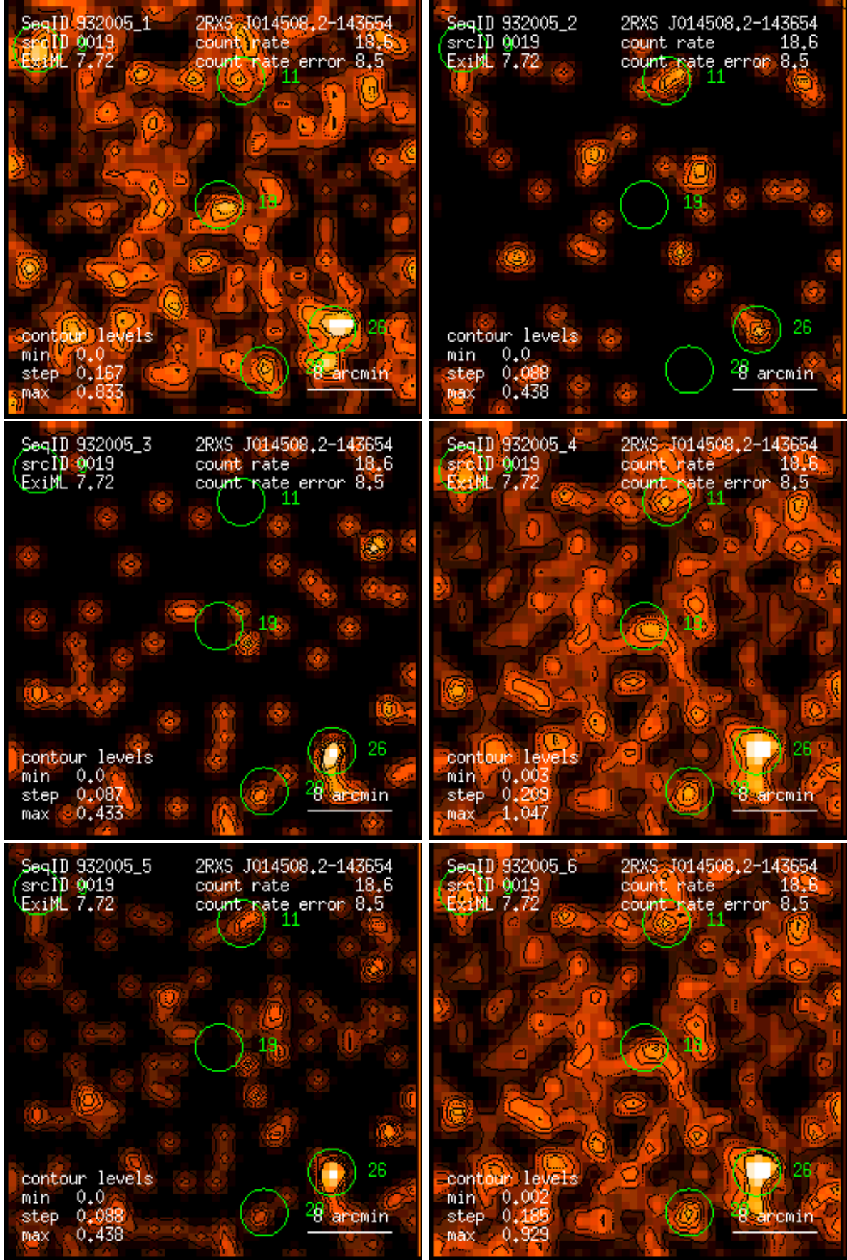
Figure 19: RASS 932005: detection 0019: band rate images, Gaussian filter: (1) PSPC channels 11 – 41, (2) 52 – 90, (3) 91 – 201, (4) 11 – 235, (5) 52 – 201, (6) 11 – 201. Broad band rates in counts/ks. Band rate contour levels in counts/ks/arcmin 2 .
