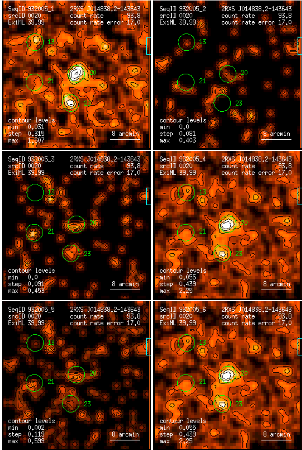
Figure 20: RASS 932005: detection 0020: band rate images, Gaussian filter: (1) PSPC channels 11 – 41, (2) 52 – 90, (3) 91 – 201, (4) 11 – 235, (5) 52 – 201, (6) 11 – 201. Broad band rates in counts/ks. Band rate contour levels in counts/ks/arcmin 2 .
