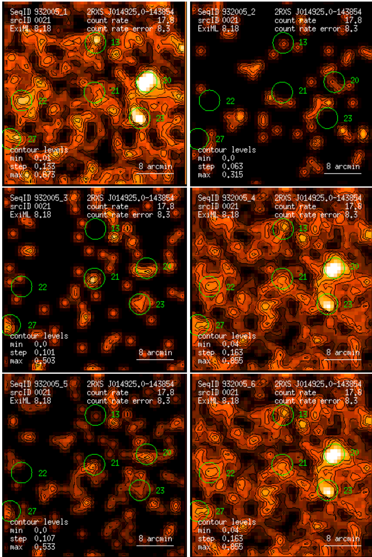
Figure 21: RASS 932005: detection 0021: band rate images, Gaussian filter: (1) PSPC channels 11 – 41, (2) 52 – 90, (3) 91 – 201, (4) 11 – 235, (5) 52 – 201, (6) 11 – 201. Broad band rates in counts/ks. Band rate contour levels in counts/ks/arcmin 2 .
