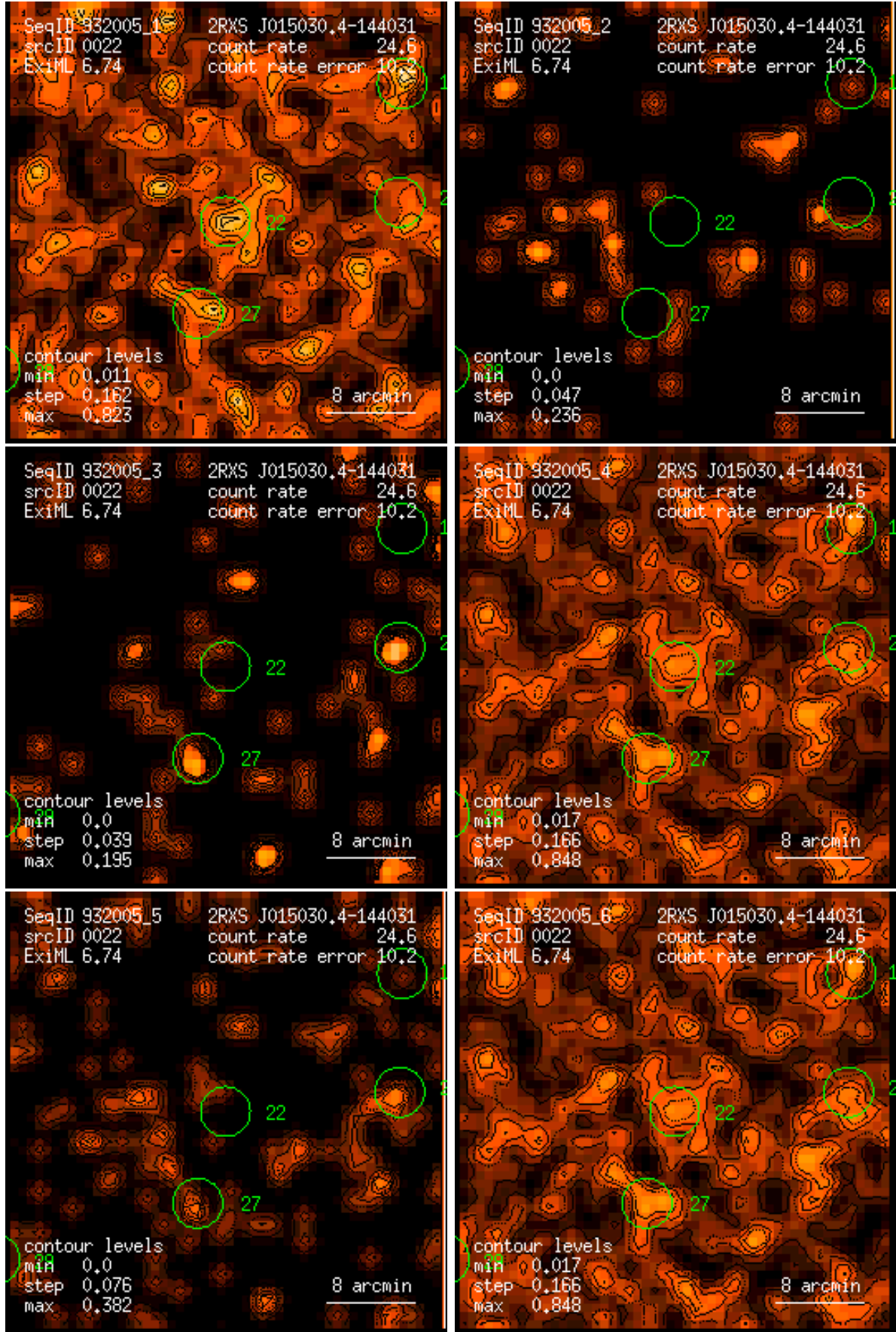
Figure 22: RASS 932005: detection 0022: band rate images, Gaussian filter: (1) PSPC channels 11 – 41, (2) 52 – 90, (3) 91 – 201, (4) 11 – 235, (5) 52 – 201, (6) 11 – 201. Broad band rates in counts/ks. Band rate contour levels in counts/ks/arcmin 2 .
