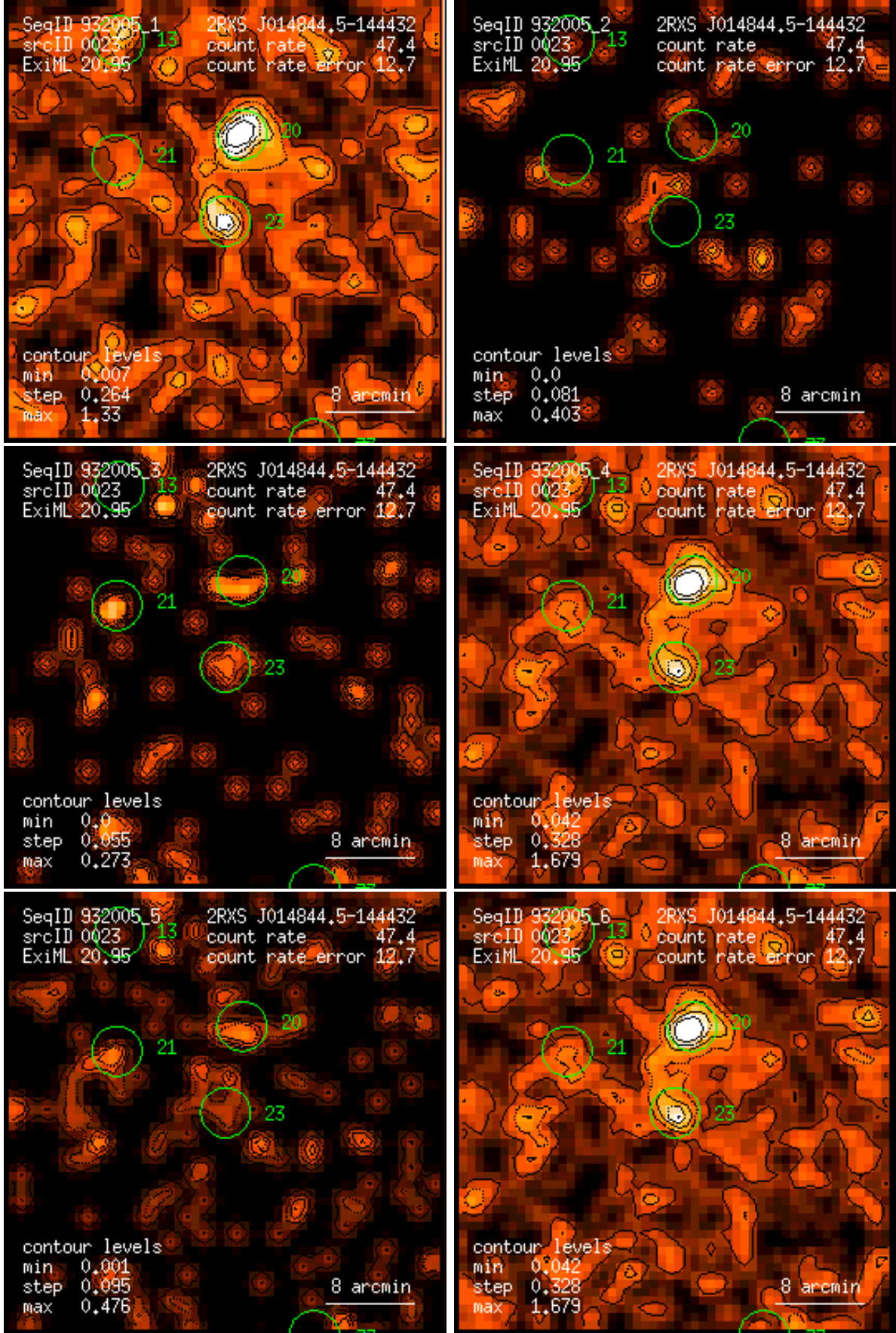
Figure 23: RASS 932005: detection 0023: band rate images, Gaussian filter: (1) PSPC channels 11 – 41, (2) 52 – 90, (3) 91 – 201, (4) 11 – 235, (5) 52 – 201, (6) 11 – 201. Broad band rates in counts/ks. Band rate contour levels in counts/ks/arcmin 2 .
