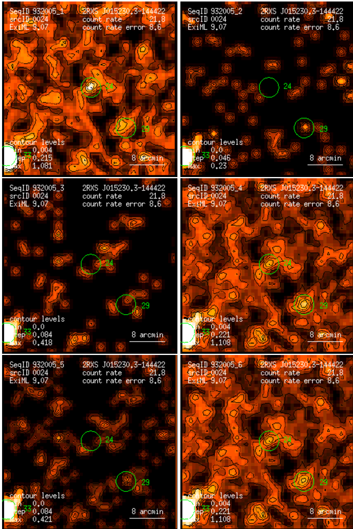
Figure 24: RASS 932005: detection 0024: band rate images, Gaussian filter: (1) PSPC channels 11 – 41, (2) 52 – 90, (3) 91 – 201, (4) 11 – 235, (5) 52 – 201, (6) 11 – 201. Broad band rates in counts/ks. Band rate contour levels in counts/ks/arcmin 2 .
