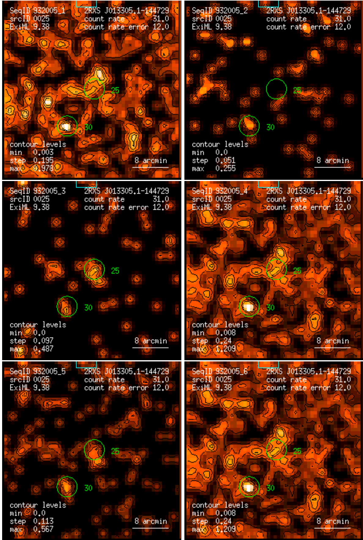
Figure 25: RASS 932005: detection 0025: band rate images, Gaussian filter: (1) PSPC channels 11 – 41, (2) 52 – 90, (3) 91 – 201, (4) 11 – 235, (5) 52 – 201, (6) 11 – 201. Broad band rates in counts/ks. Band rate contour levels in counts/ks/arcmin 2 .
