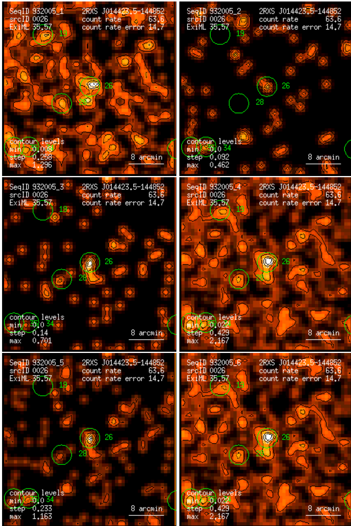
Figure 26: RASS 932005: detection 0026: band rate images, Gaussian filter: (1) PSPC channels 11 – 41, (2) 52 – 90, (3) 91 – 201, (4) 11 – 235, (5) 52 – 201, (6) 11 – 201. Broad band rates in counts/ks. Band rate contour levels in counts/ks/arcmin 2 .
