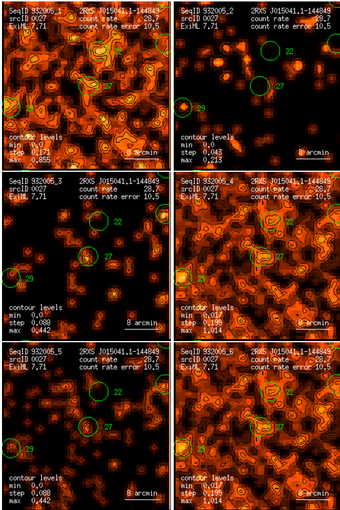
Figure 27: RASS 932005: detection 0027: band rate images, Gaussian filter: (1) PSPC channels 11 – 41, (2) 52 – 90, (3) 91 – 201, (4) 11 – 235, (5) 52 – 201, (6) 11 – 201. Broad band rates in counts/ks. Band rate contour levels in counts/ks/arcmin 2 .
