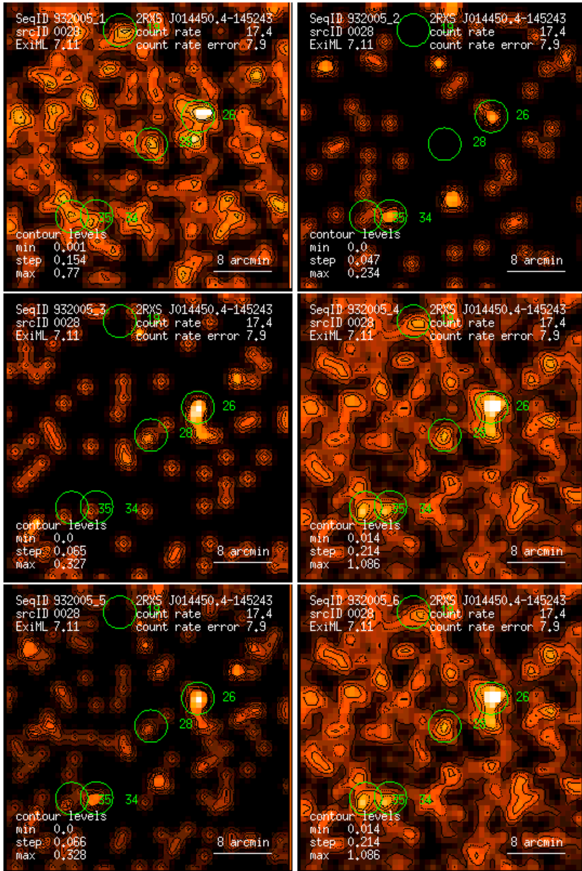
Figure 28: RASS 932005: detection 0028: band rate images, Gaussian filter: (1) PSPC channels 11 – 41, (2) 52 – 90, (3) 91 – 201, (4) 11 – 235, (5) 52 – 201, (6) 11 – 201. Broad band rates in counts/ks. Band rate contour levels in counts/ks/arcmin 2 .
