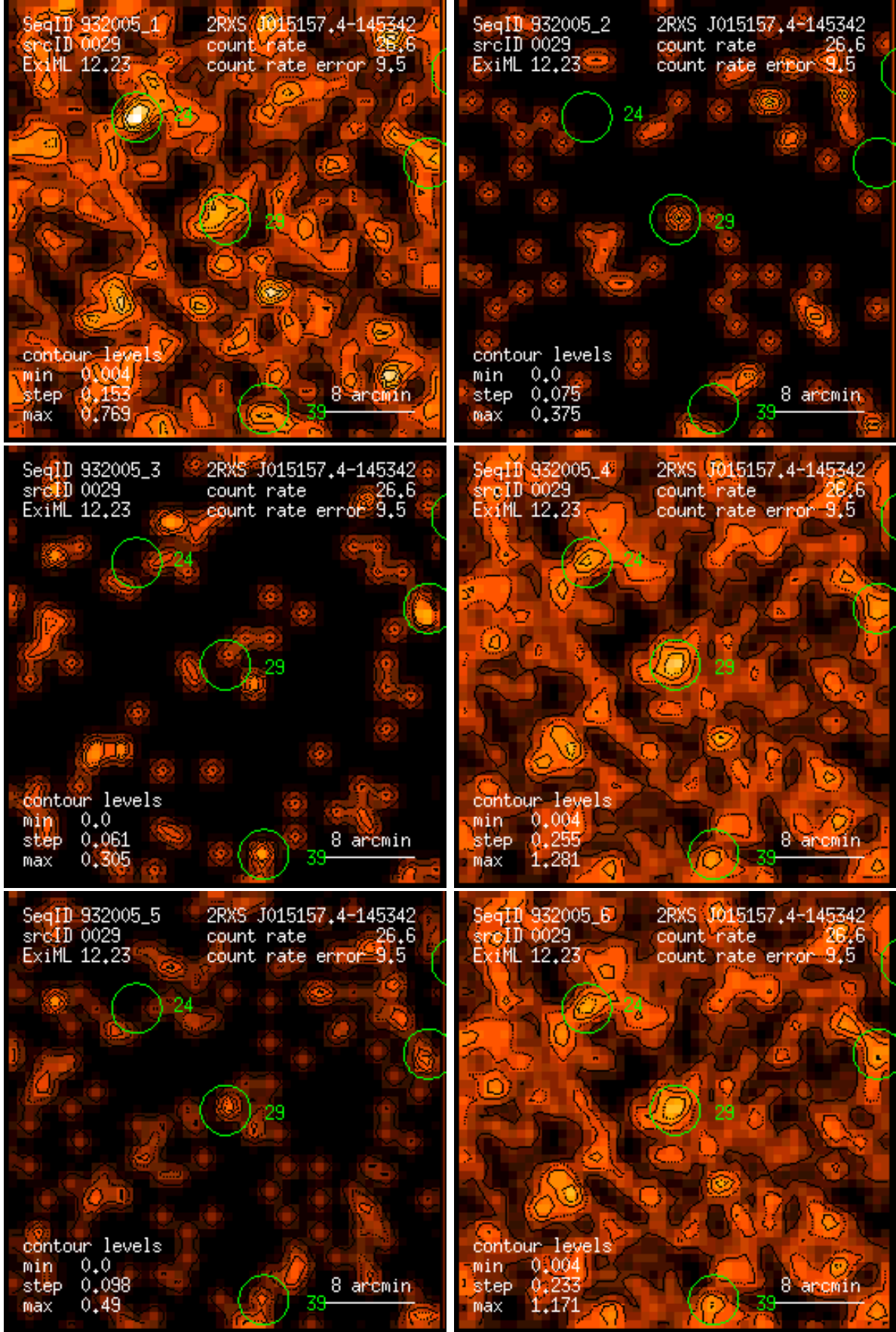
Figure 29: RASS 932005: detection 0029: band rate images, Gaussian filter: (1) PSPC channels 11 – 41, (2) 52 – 90, (3) 91 – 201, (4) 11 – 235, (5) 52 – 201, (6) 11 – 201. Broad band rates in counts/ks. Band rate contour levels in counts/ks/arcmin 2 .
