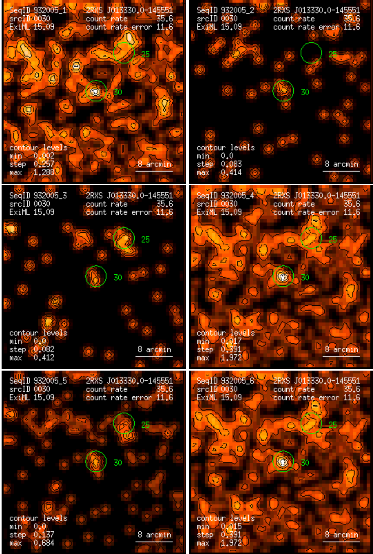
Figure 30: RASS 932005: detection 0030: band rate images, Gaussian filter: (1) PSPC channels 11 – 41, (2) 52 – 90, (3) 91 – 201, (4) 11 – 235, (5) 52 – 201, (6) 11 – 201. Broad band rates in counts/ks. Band rate contour levels in counts/ks/arcmin 2 .
