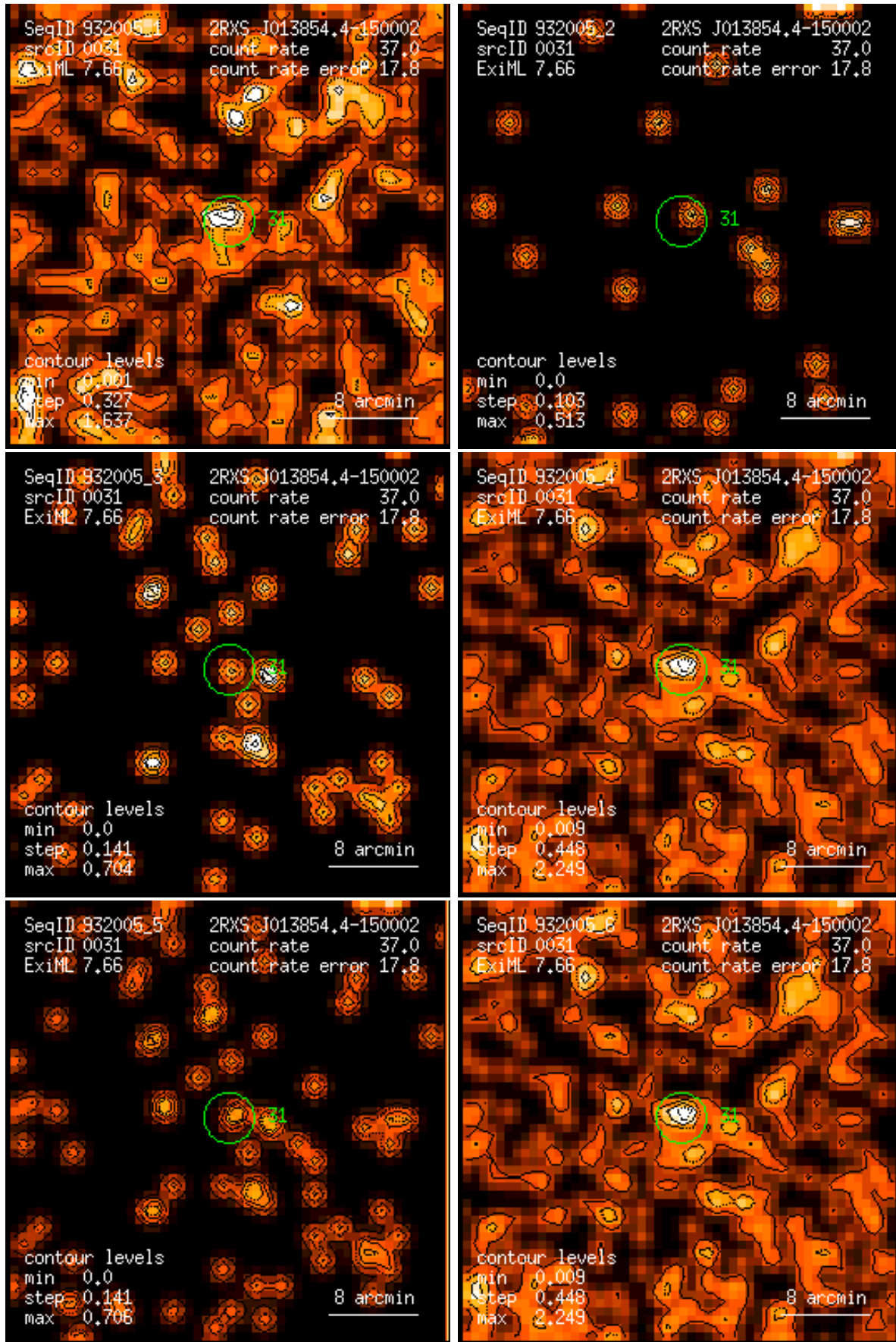
Figure 31: RASS 932005: detection 0031: band rate images, Gaussian filter: (1) PSPC channels 11 – 41, (2) 52 – 90, (3) 91 – 201, (4) 11 – 235, (5) 52 – 201, (6) 11 – 201. Broad band rates in counts/ks. Band rate contour levels in counts/ks/arcmin 2 .
