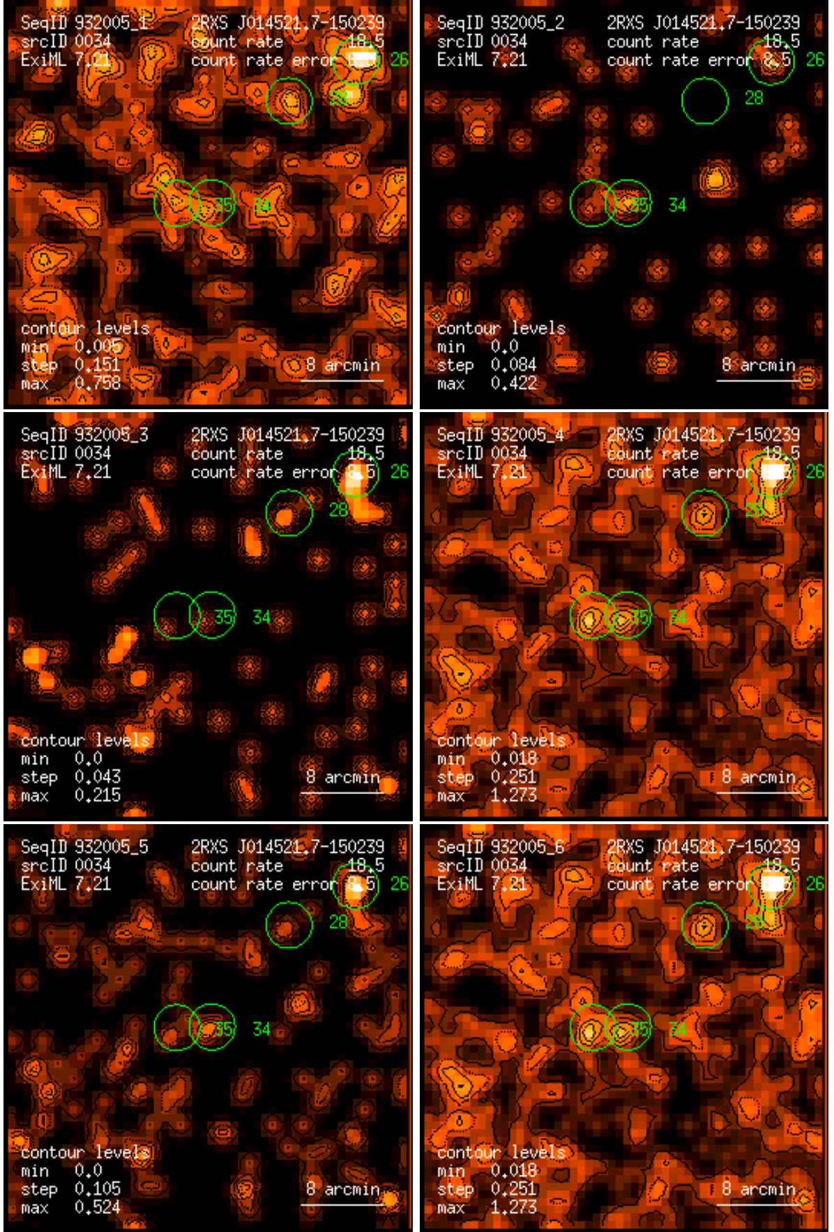
Figure 34: RASS 932005: detection 0034: band rate images, Gaussian filter: (1) PSPC channels 11 – 41, (2) 52 – 90, (3) 91 – 201, (4) 11 – 235, (5) 52 – 201, (6) 11 – 201. Broad band rates in counts/ks. Band rate contour levels in counts/ks/arcmin 2 .
