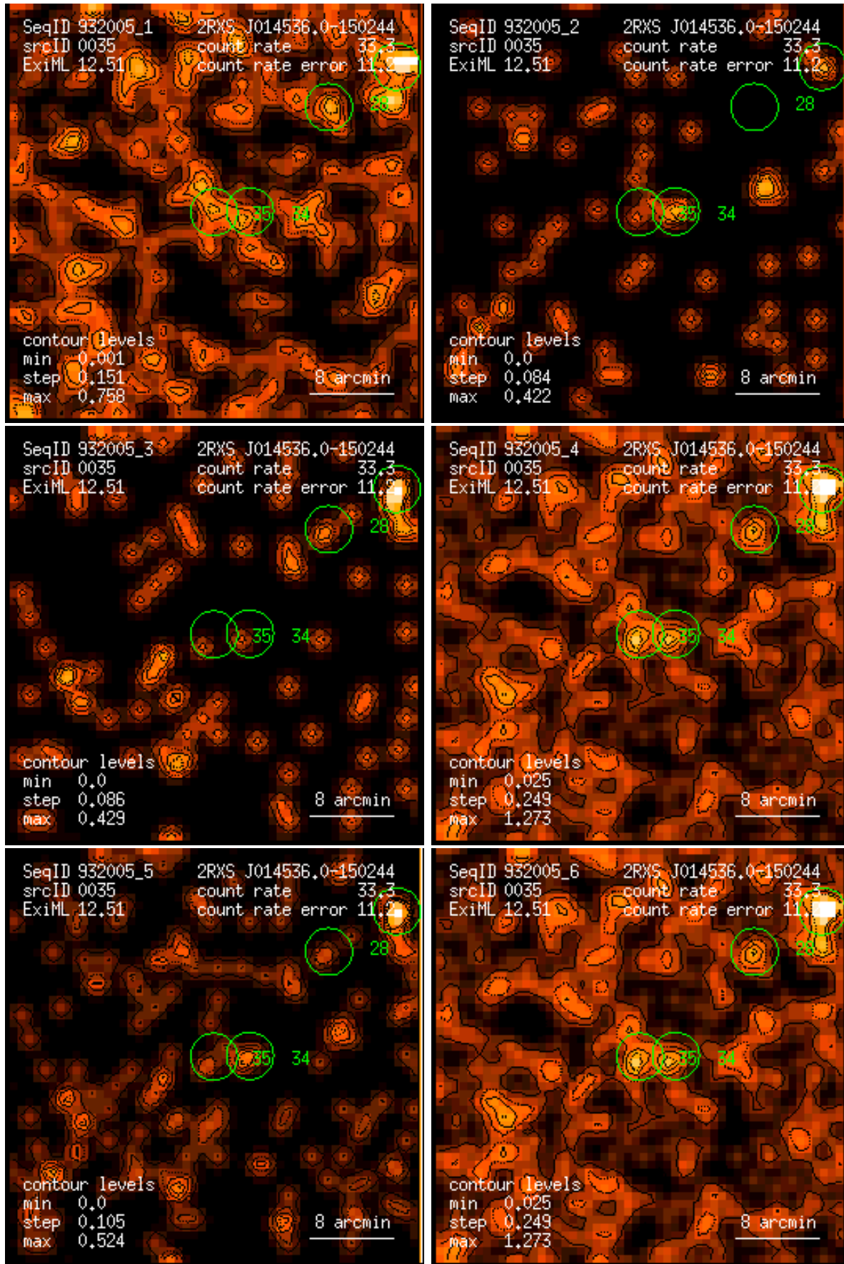
Figure 35: RASS 932005: detection 0035: band rate images, Gaussian filter: (1) PSPC channels 11 – 41, (2) 52 – 90, (3) 91 – 201, (4) 11 – 235, (5) 52 – 201, (6) 11 – 201. Broad band rates in counts/ks. Band rate contour levels in counts/ks/arcmin 2 .
