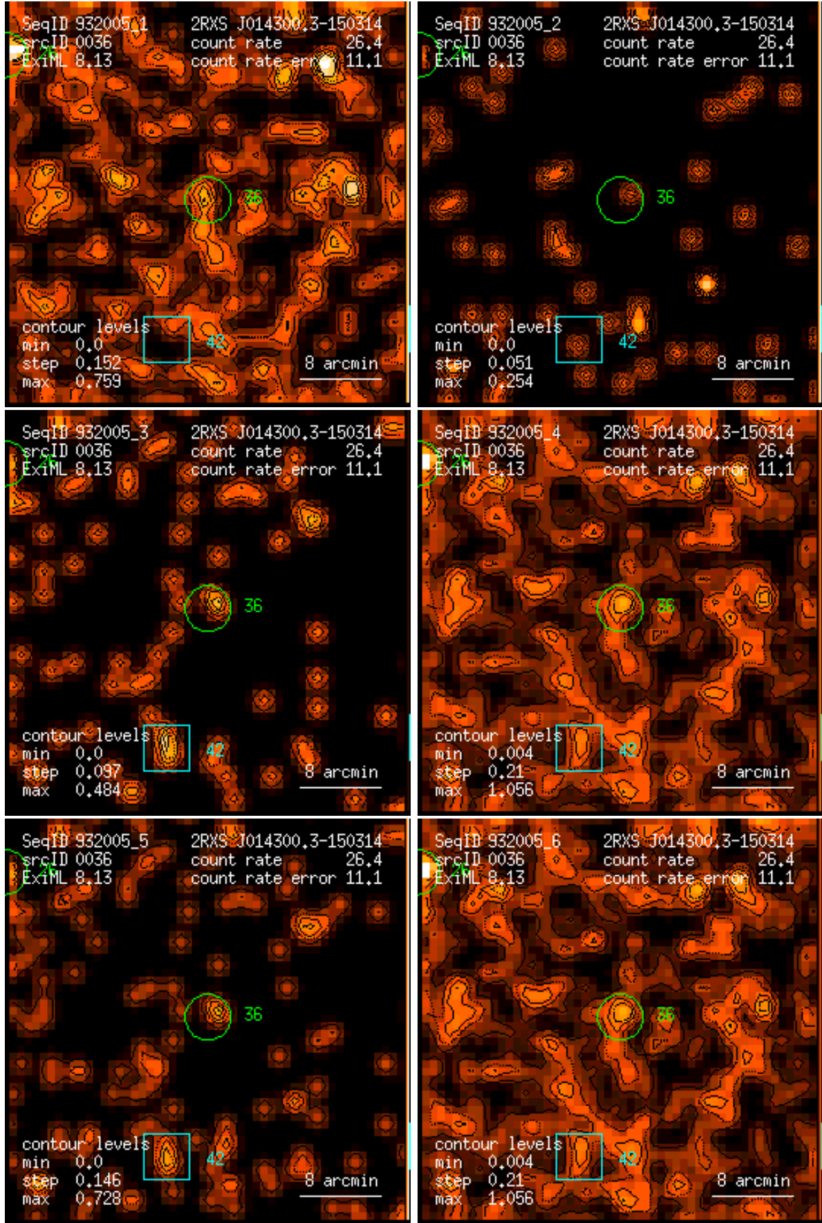
Figure 36: RASS 932005: detection 0036: band rate images, Gaussian filter: (1) PSPC channels 11 – 41, (2) 52 – 90, (3) 91 – 201, (4) 11 – 235, (5) 52 – 201, (6) 11 – 201. Broad band rates in counts/ks. Band rate contour levels in counts/ks/arcmin 2 .
