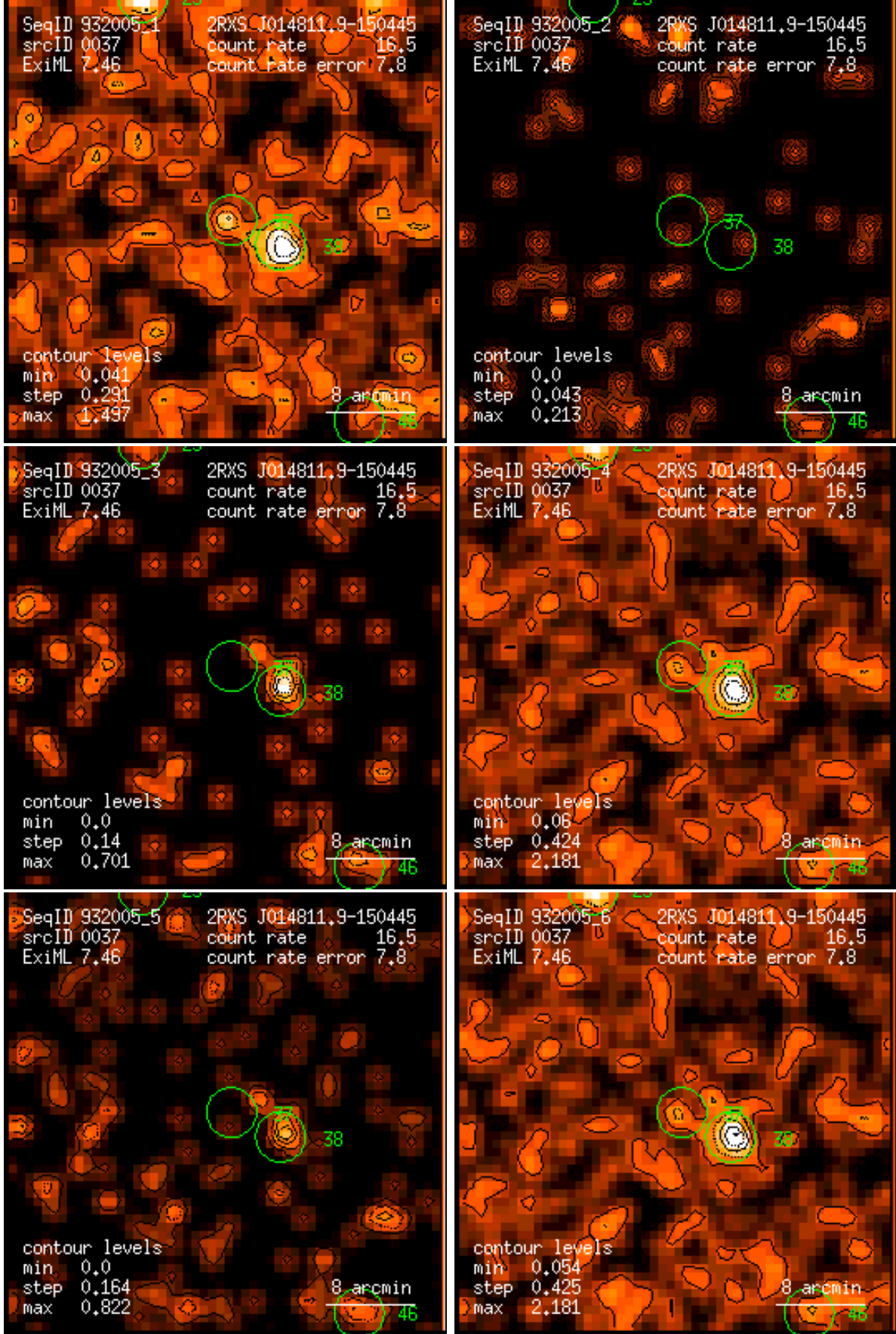
Figure 37: RASS 932005: detection 0037: band rate images, Gaussian filter: (1) PSPC channels 11 – 41, (2) 52 – 90, (3) 91 – 201, (4) 11 – 235, (5) 52 – 201, (6) 11 – 201. Broad band rates in counts/ks. Band rate contour levels in counts/ks/arcmin 2 .
