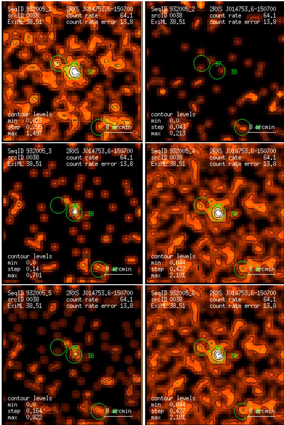
Figure 38: RASS 932005: detection 0038: band rate images, Gaussian filter: (1) PSPC channels 11 – 41, (2) 52 – 90, (3) 91 – 201, (4) 11 – 235, (5) 52 – 201, (6) 11 – 201. Broad band rates in counts/ks. Band rate contour levels in counts/ks/arcmin 2 .
