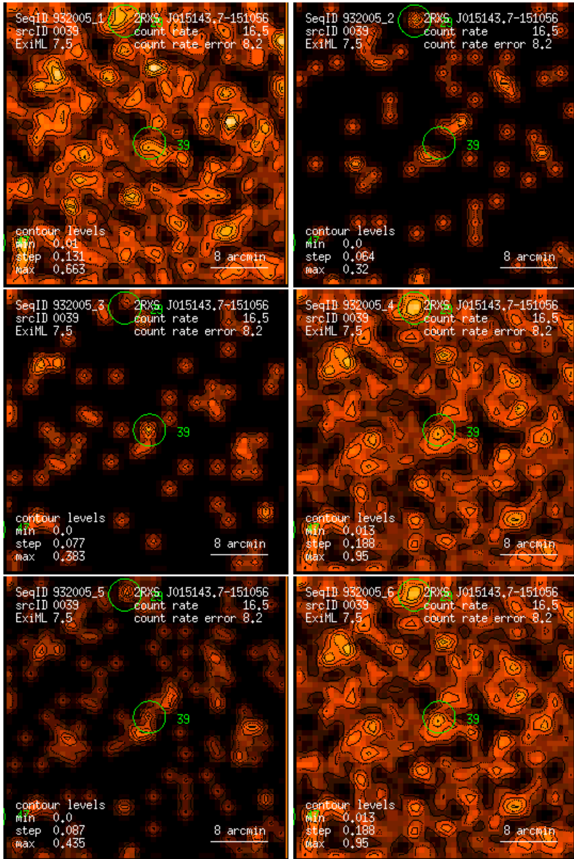
Figure 39: RASS 932005: detection 0039: band rate images, Gaussian filter: (1) PSPC channels 11 – 41, (2) 52 – 90, (3) 91 – 201, (4) 11 – 235, (5) 52 – 201, (6) 11 – 201. Broad band rates in counts/ks. Band rate contour levels in counts/ks/arcmin 2 .
