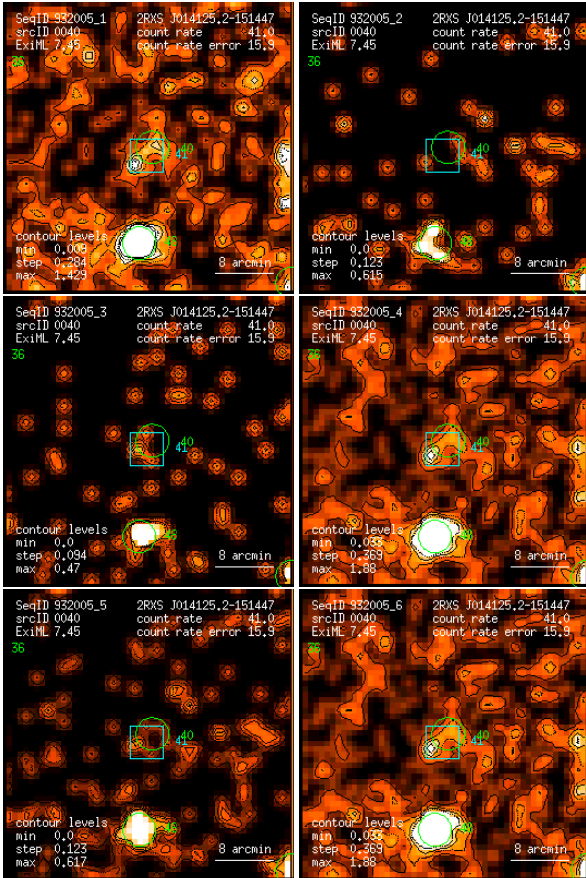
Figure 40: RASS 932005: detection 0040: band rate images, Gaussian filter: (1) PSPC channels 11 – 41, (2) 52 – 90, (3) 91 – 201, (4) 11 – 235, (5) 52 – 201, (6) 11 – 201. Broad band rates in counts/ks. Band rate contour levels in counts/ks/arcmin 2 .
