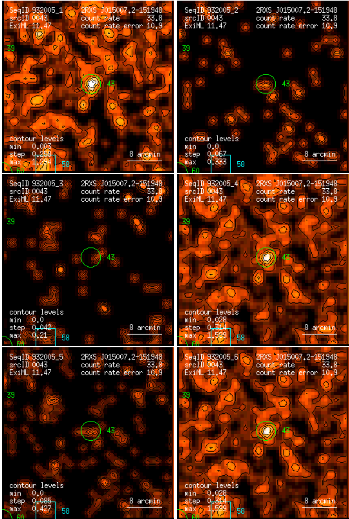
Figure 43: RASS 932005: detection 0043: band rate images, Gaussian filter: (1) PSPC channels 11 – 41, (2) 52 – 90, (3) 91 – 201, (4) 11 – 235, (5) 52 – 201, (6) 11 – 201. Broad band rates in counts/ks. Band rate contour levels in counts/ks/arcmin 2 .
