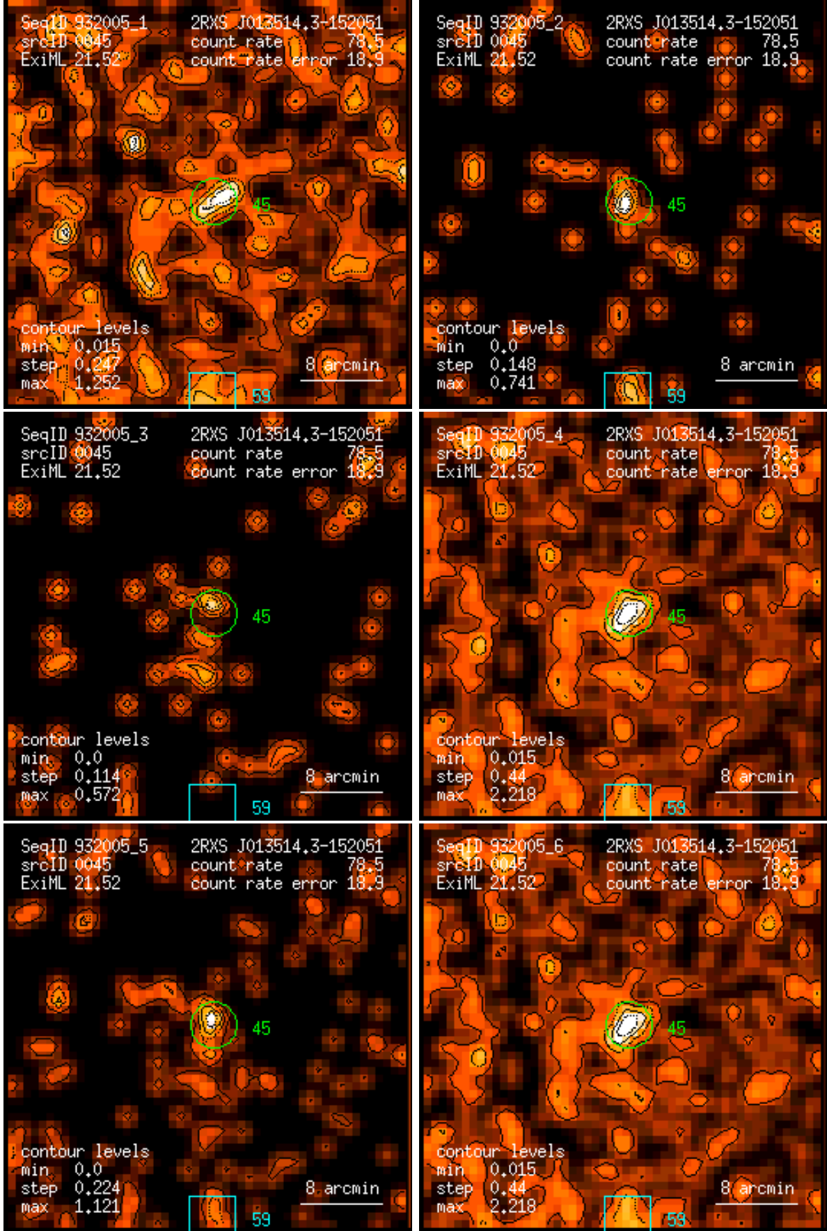
Figure 45: RASS 932005: detection 0045: band rate images, Gaussian filter: (1) PSPC channels 11 – 41, (2) 52 – 90, (3) 91 – 201, (4) 11 – 235, (5) 52 – 201, (6) 11 – 201. Broad band rates in counts/ks. Band rate contour levels in counts/ks/arcmin 2 .
