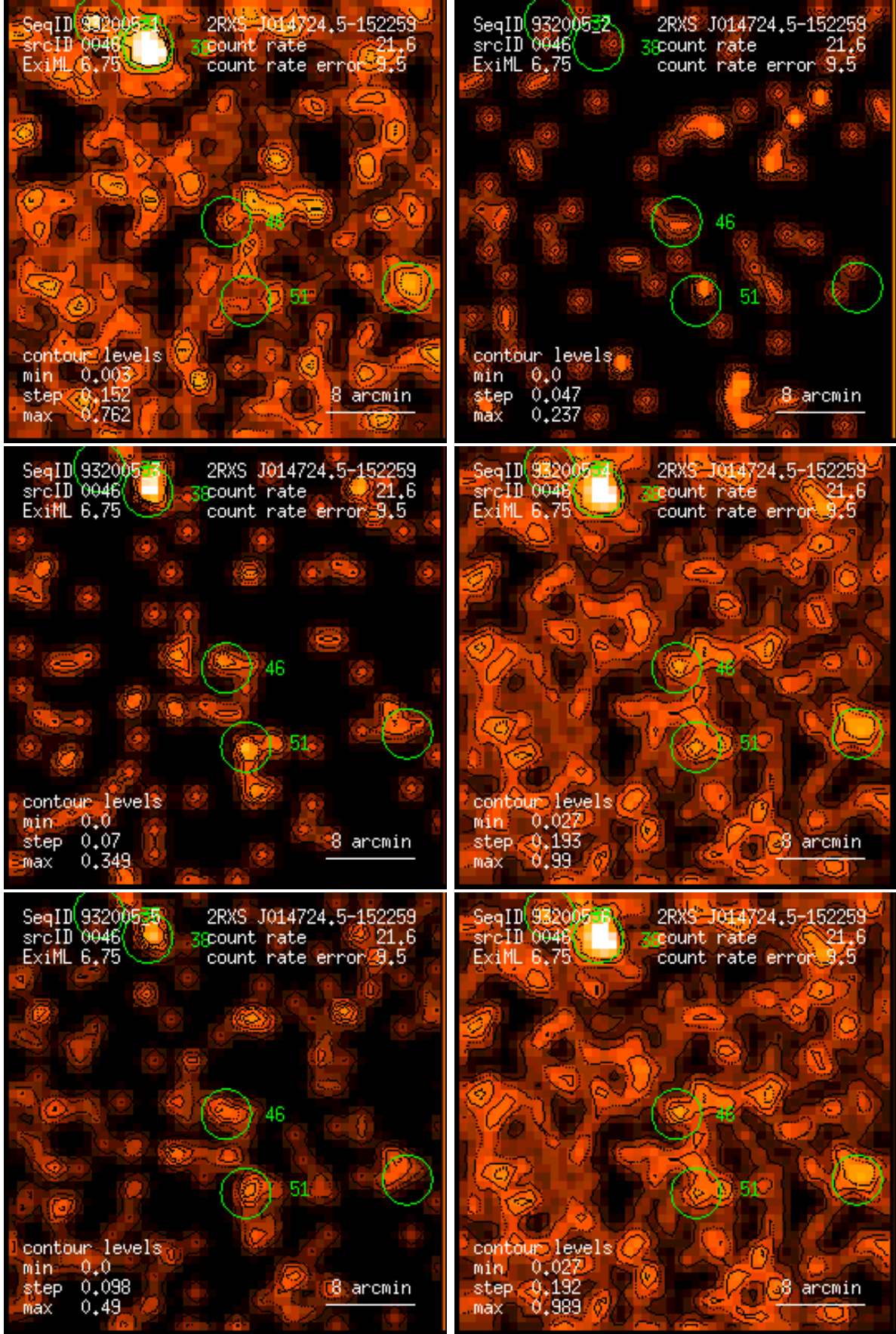
Figure 46: RASS 932005: detection 0046: band rate images, Gaussian filter: (1) PSPC channels 11 – 41, (2) 52 – 90, (3) 91 – 201, (4) 11 – 235, (5) 52 – 201, (6) 11 – 201. Broad band rates in counts/ks. Band rate contour levels in counts/ks/arcmin 2 .
