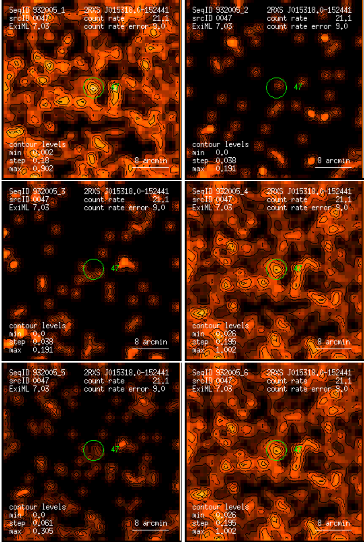
Figure 47: RASS 932005: detection 0047: band rate images, Gaussian filter: (1) PSPC channels 11 – 41, (2) 52 – 90, (3) 91 – 201, (4) 11 – 235, (5) 52 – 201, (6) 11 – 201. Broad band rates in counts/ks. Band rate contour levels in counts/ks/arcmin 2 .
