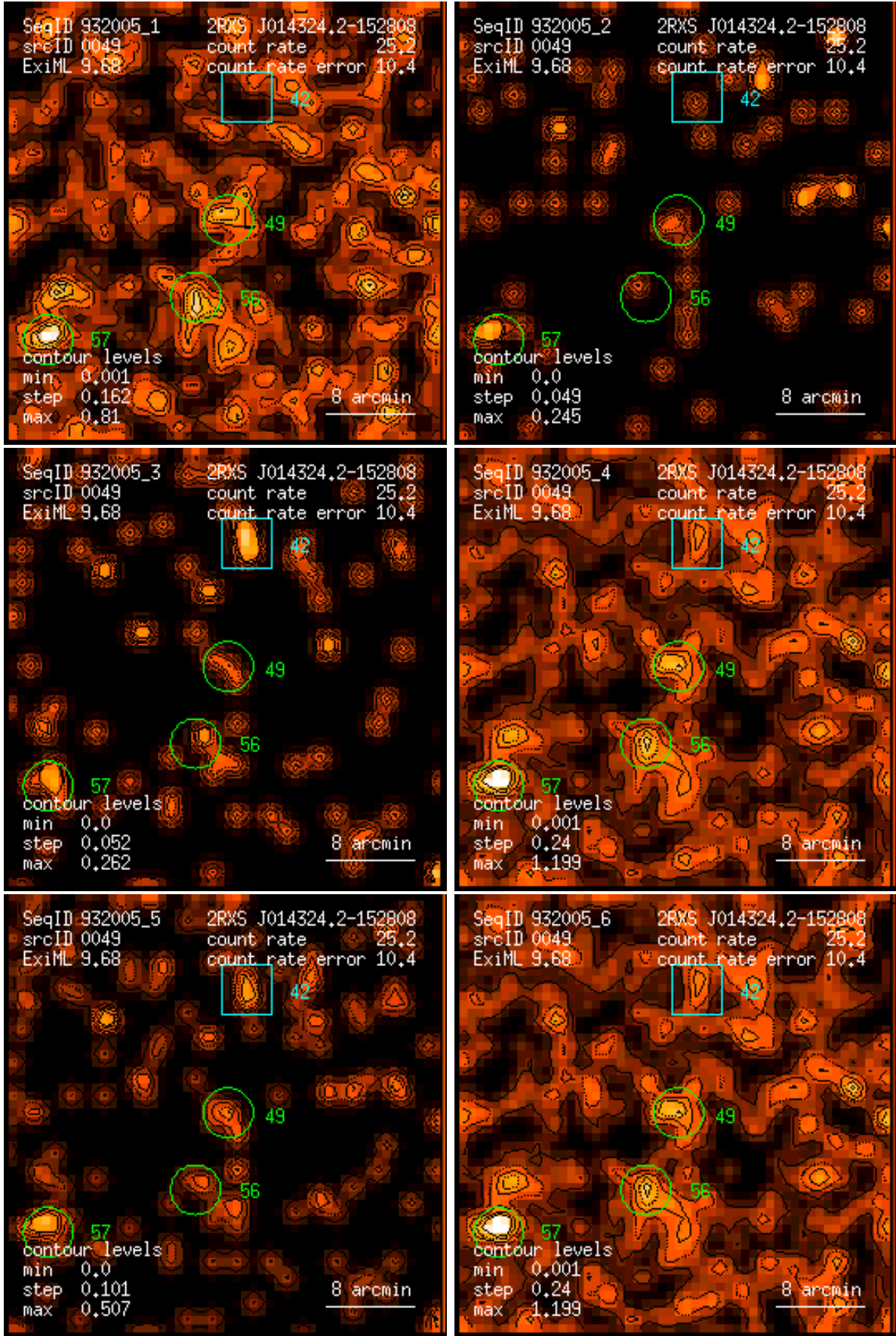
Figure 49: RASS 932005: detection 0049: band rate images, Gaussian filter: (1) PSPC channels 11 – 41, (2) 52 – 90, (3) 91 – 201, (4) 11 – 235, (5) 52 – 201, (6) 11 – 201. Broad band rates in counts/ks. Band rate contour levels in counts/ks/arcmin 2 .
