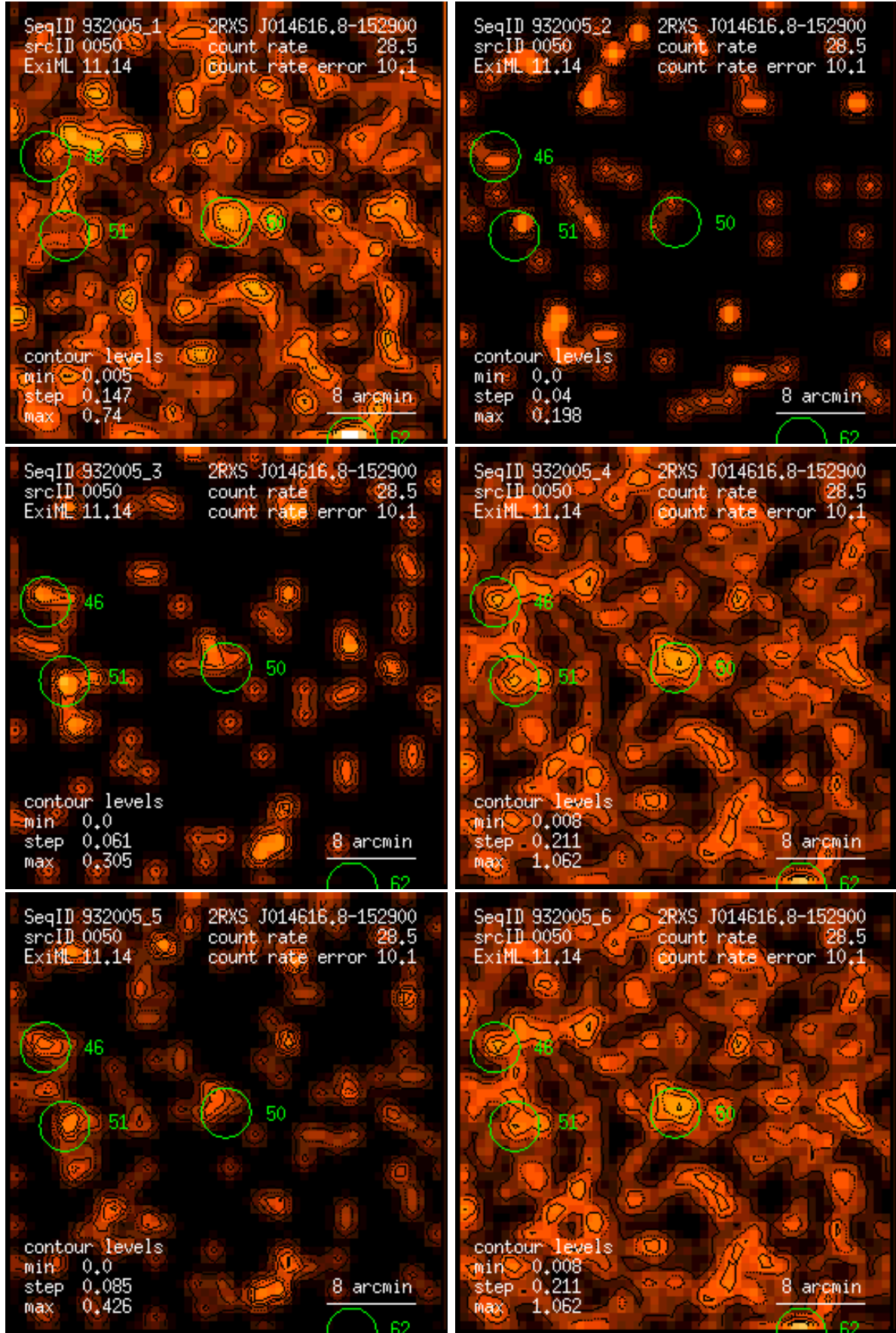
Figure 50: RASS 932005: detection 0050: band rate images, Gaussian filter: (1) PSPC channels 11 – 41, (2) 52 – 90, (3) 91 – 201, (4) 11 – 235, (5) 52 – 201, (6) 11 – 201. Broad band rates in counts/ks. Band rate contour levels in counts/ks/arcmin 2 .
