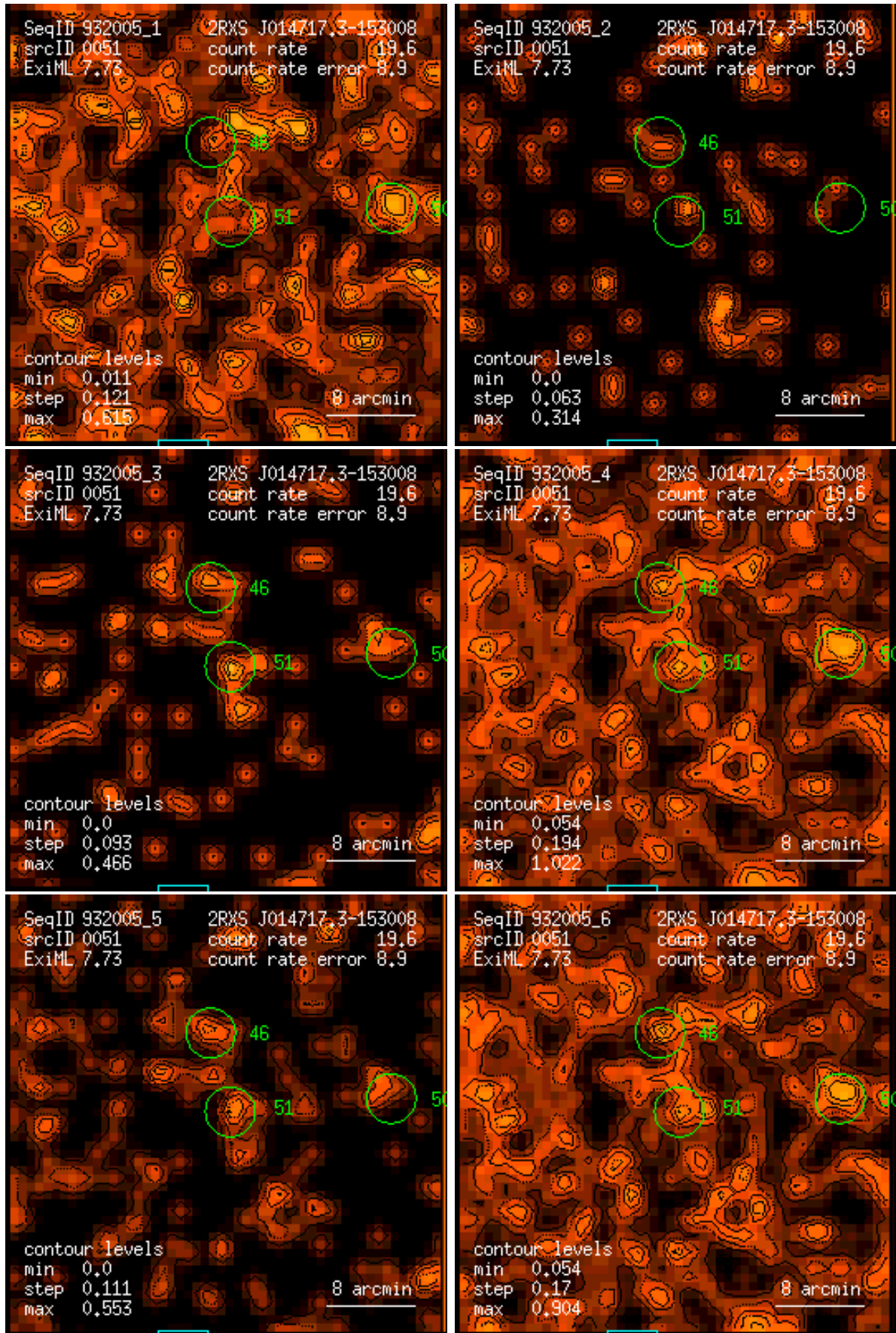
Figure 51: RASS 932005: detection 0051: band rate images, Gaussian filter: (1) PSPC channels 11 – 41, (2) 52 – 90, (3) 91 – 201, (4) 11 – 235, (5) 52 – 201, (6) 11 – 201. Broad band rates in counts/ks. Band rate contour levels in counts/ks/arcmin 2 .
