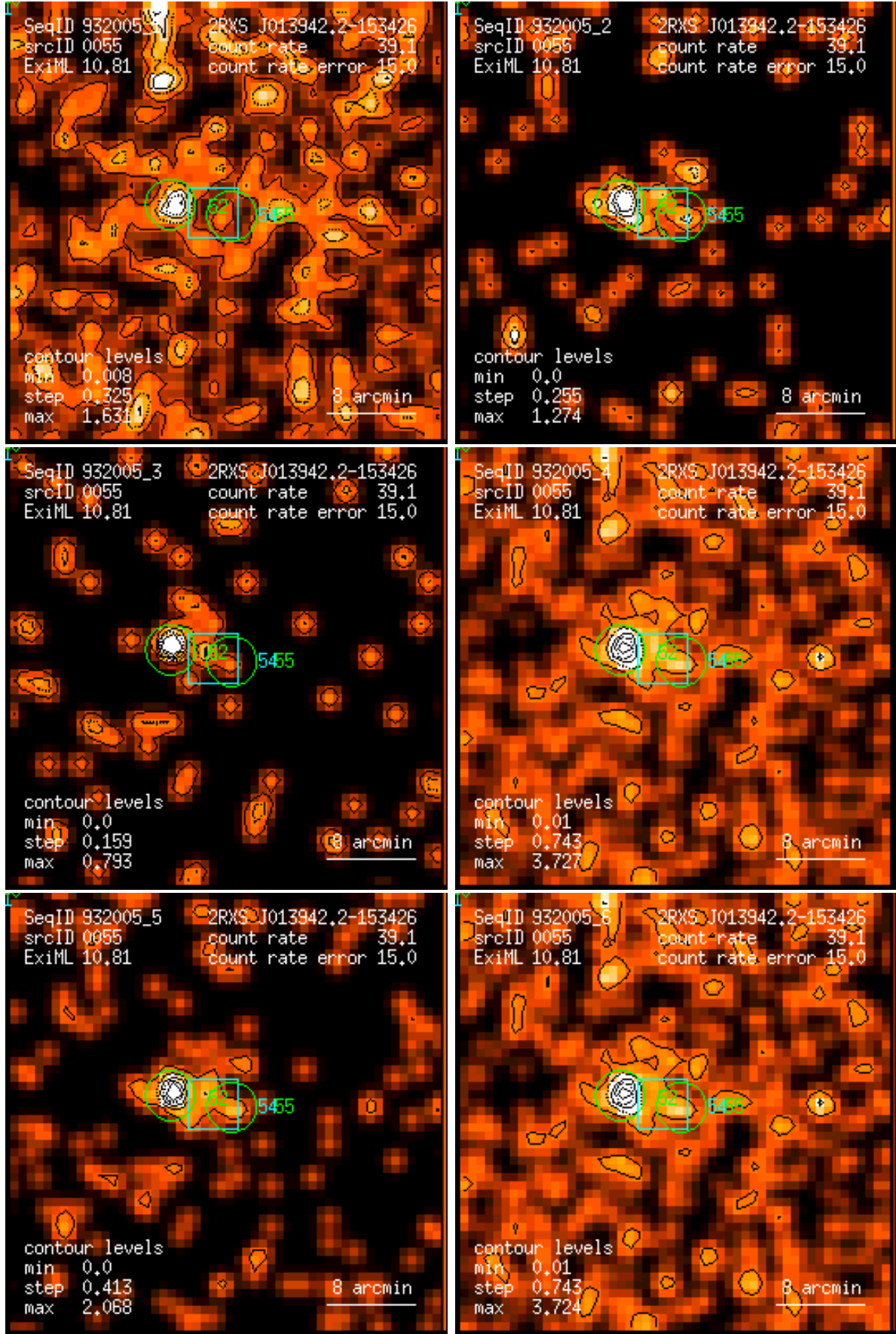
Figure 55: RASS 932005: detection 0055: band rate images, Gaussian filter: (1) PSPC channels 11 – 41, (2) 52 – 90, (3) 91 – 201, (4) 11 – 235, (5) 52 – 201, (6) 11 – 201. Broad band rates in counts/ks. Band rate contour levels in counts/ks/arcmin 2 .
