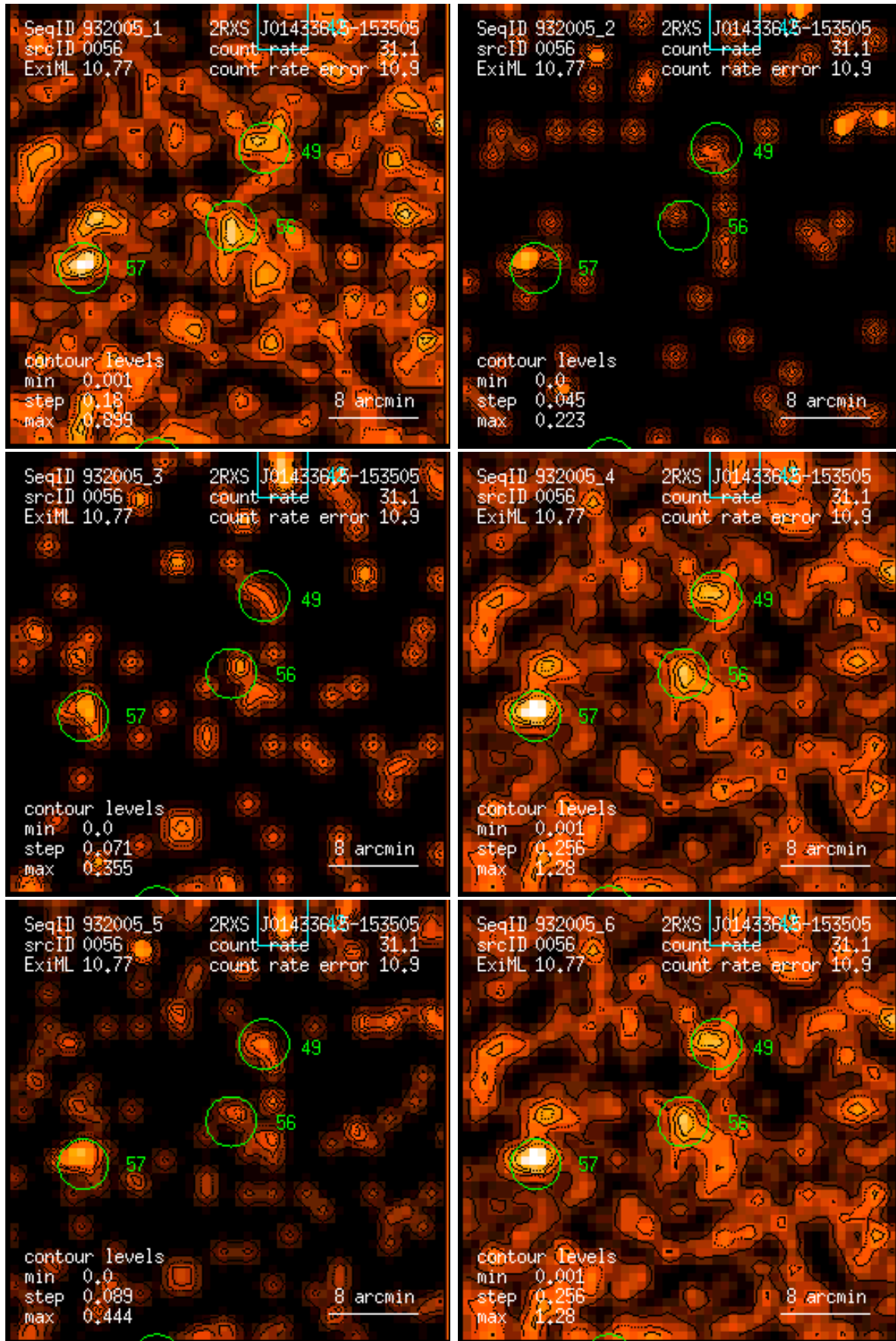
Figure 56: RASS 932005: detection 0056: band rate images, Gaussian filter: (1) PSPC channels 11 – 41, (2) 52 – 90, (3) 91 – 201, (4) 11 – 235, (5) 52 – 201, (6) 11 – 201. Broad band rates in counts/ks. Band rate contour levels in counts/ks/arcmin 2 .
