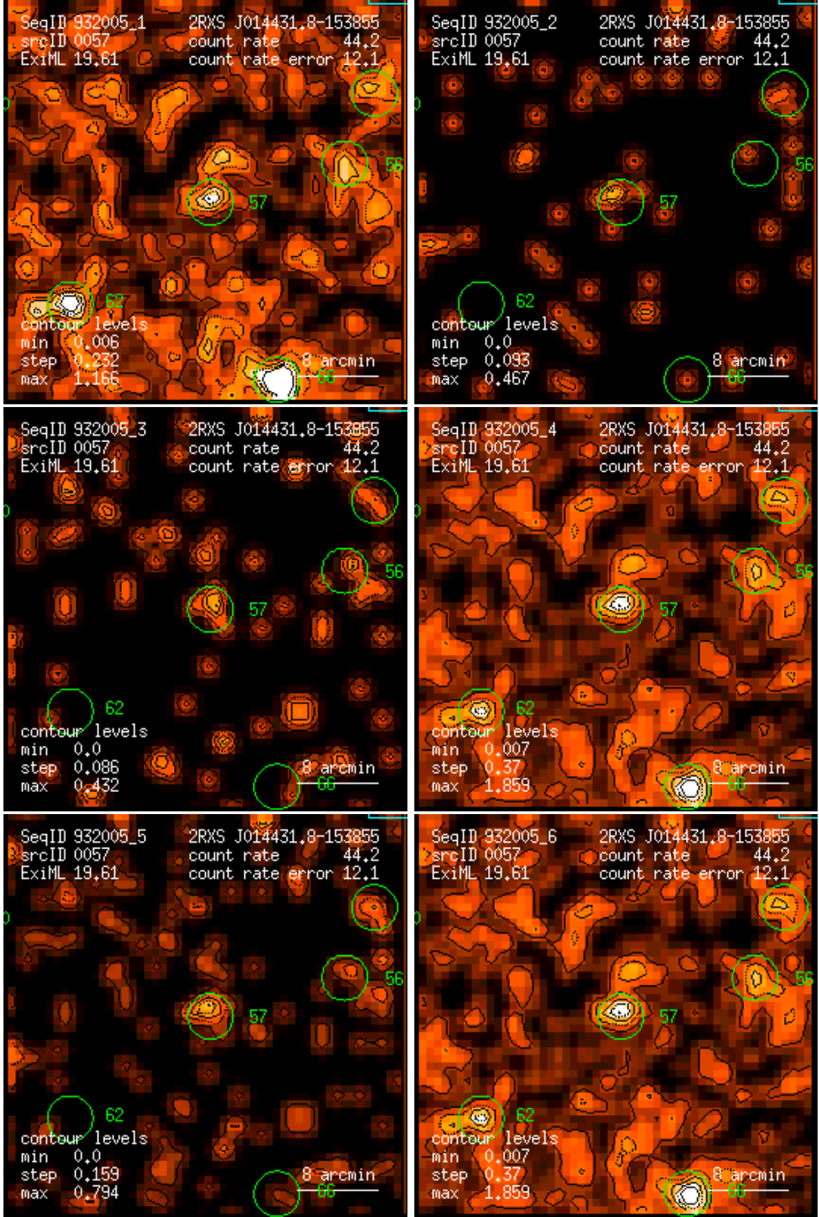
Figure 57: RASS 932005: detection 0057: band rate images, Gaussian filter: (1) PSPC channels 11 – 41, (2) 52 – 90, (3) 91 – 201, (4) 11 – 235, (5) 52 – 201, (6) 11 – 201. Broad band rates in counts/ks. Band rate contour levels in counts/ks/arcmin 2 .
