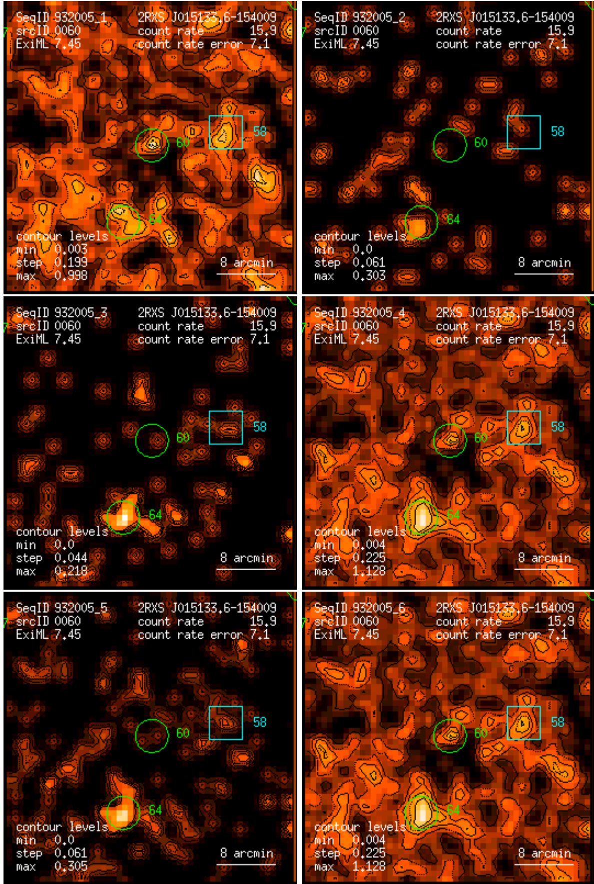
Figure 60: RASS 932005: detection 0060: band rate images, Gaussian filter: (1) PSPC channels 11 – 41, (2) 52 – 90, (3) 91 – 201, (4) 11 – 235, (5) 52 – 201, (6) 11 – 201. Broad band rates in counts/ks. Band rate contour levels in counts/ks/arcmin 2 .
