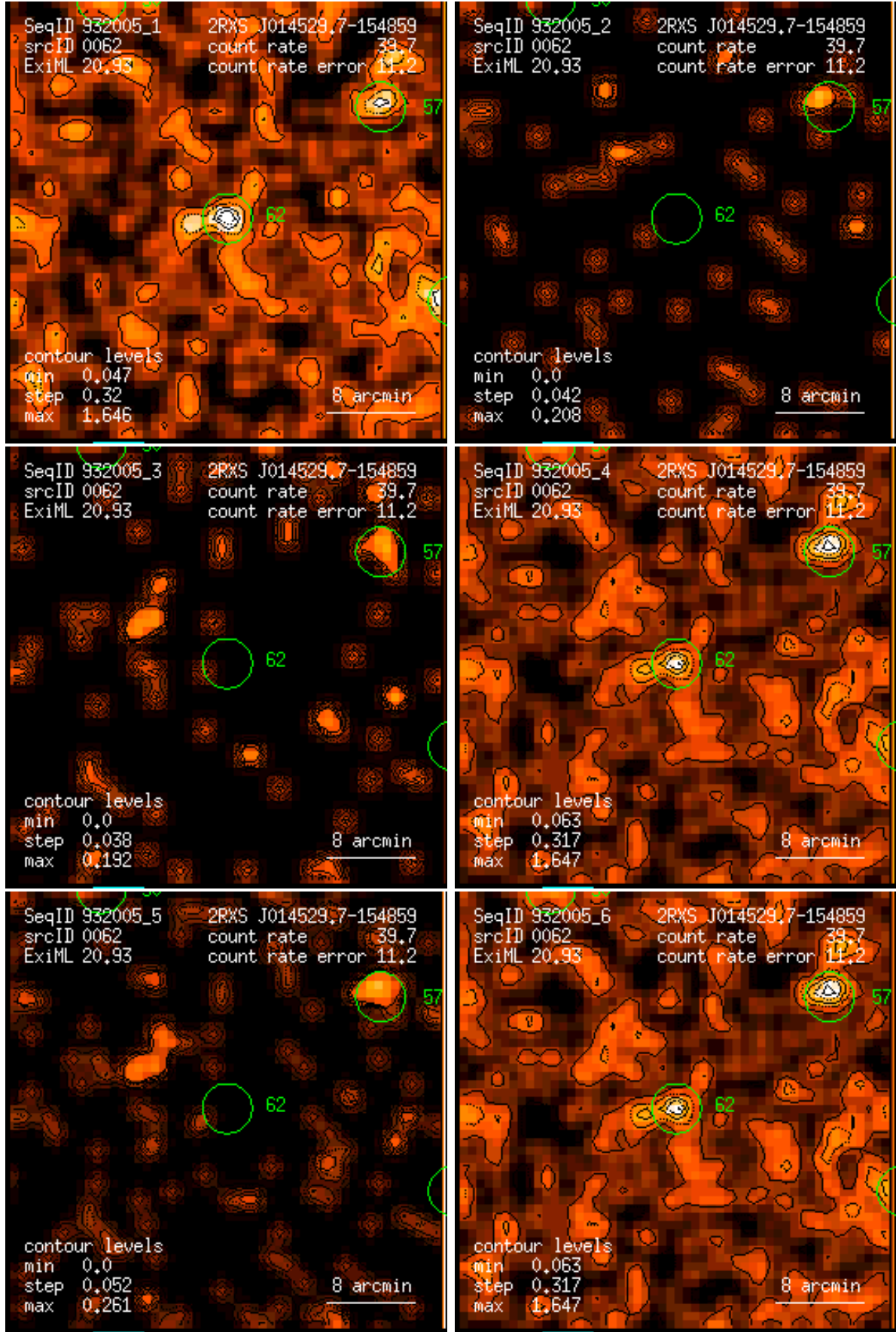
Figure 62: RASS 932005: detection 0062: band rate images, Gaussian filter: (1) PSPC channels 11 – 41, (2) 52 – 90, (3) 91 – 201, (4) 11 – 235, (5) 52 – 201, (6) 11 – 201. Broad band rates in counts/ks. Band rate contour levels in counts/ks/arcmin 2 .
